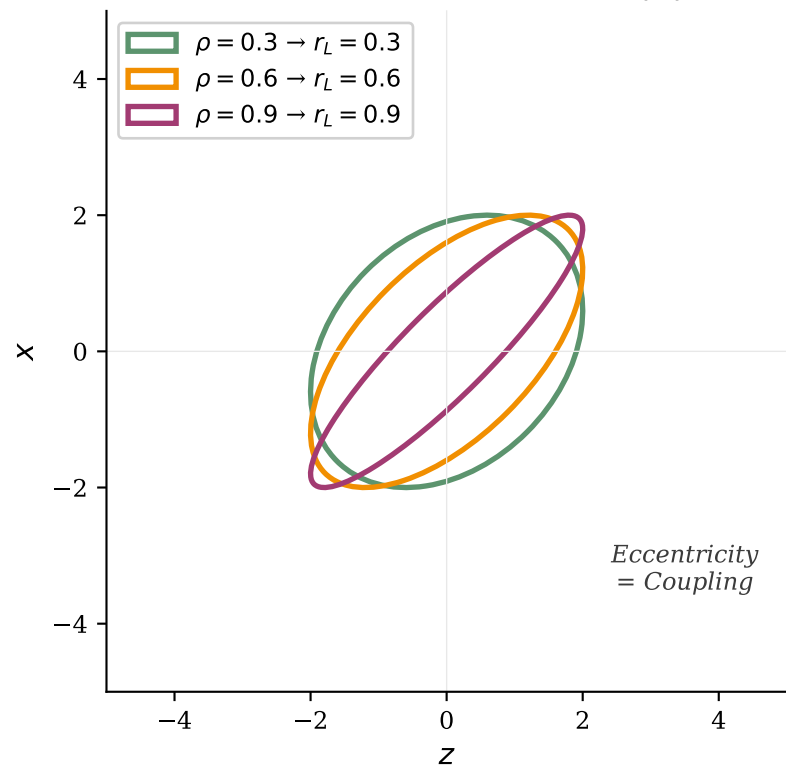
(B) Gaussian Calibration: r_L = |\rho|
