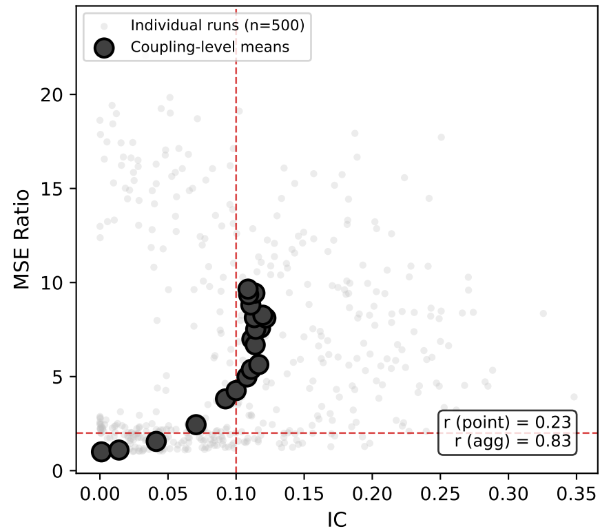
(C) IC predicts MFVI failure
