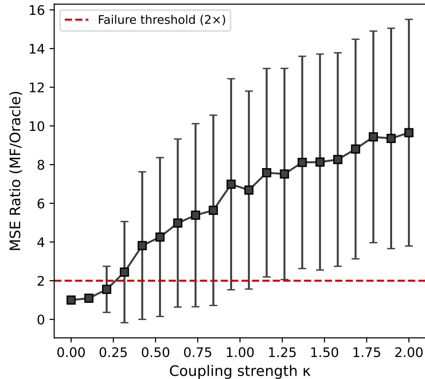
(B) MFVI degradation with coupling
