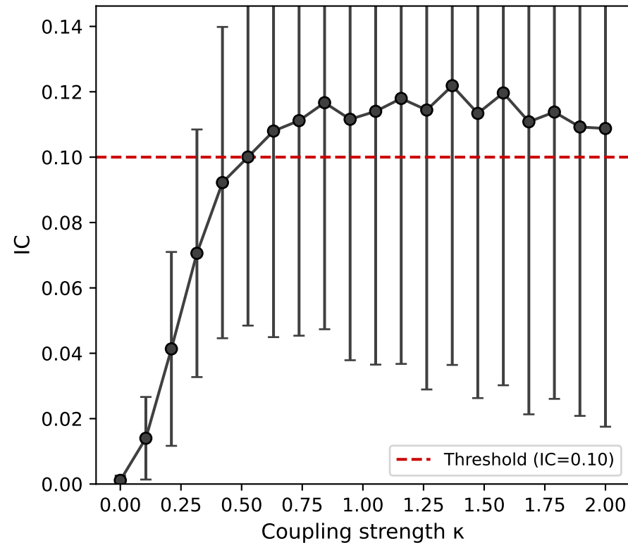
(A) IC increases with coupling
