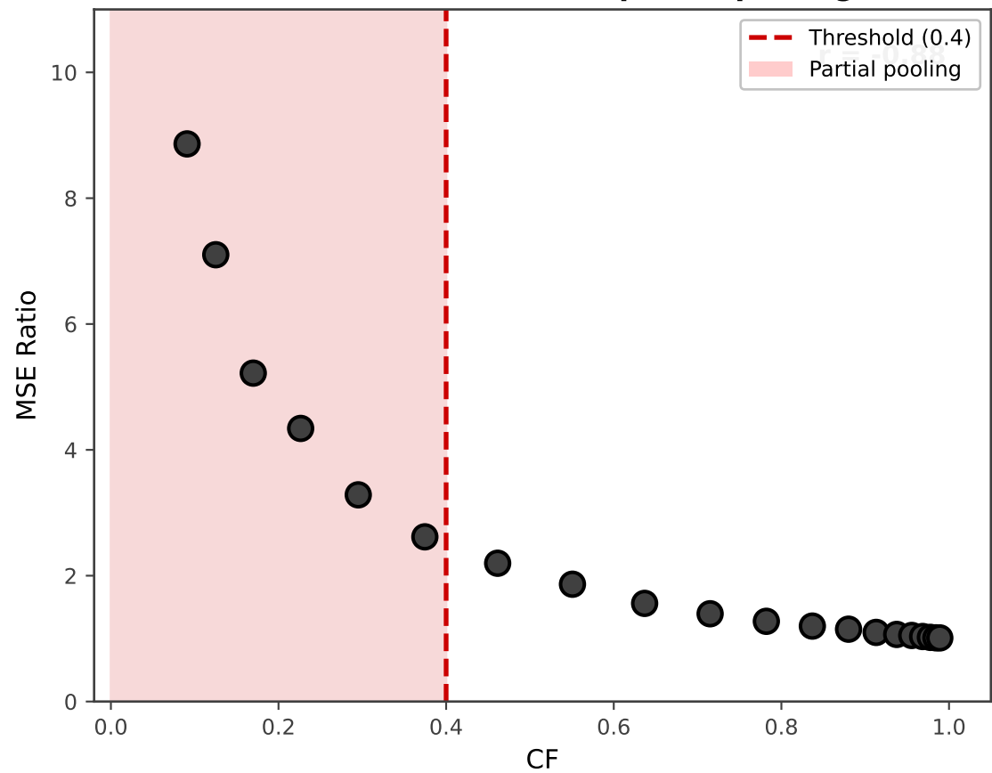
(B) HLM: Low CF -> Use partial pooling
