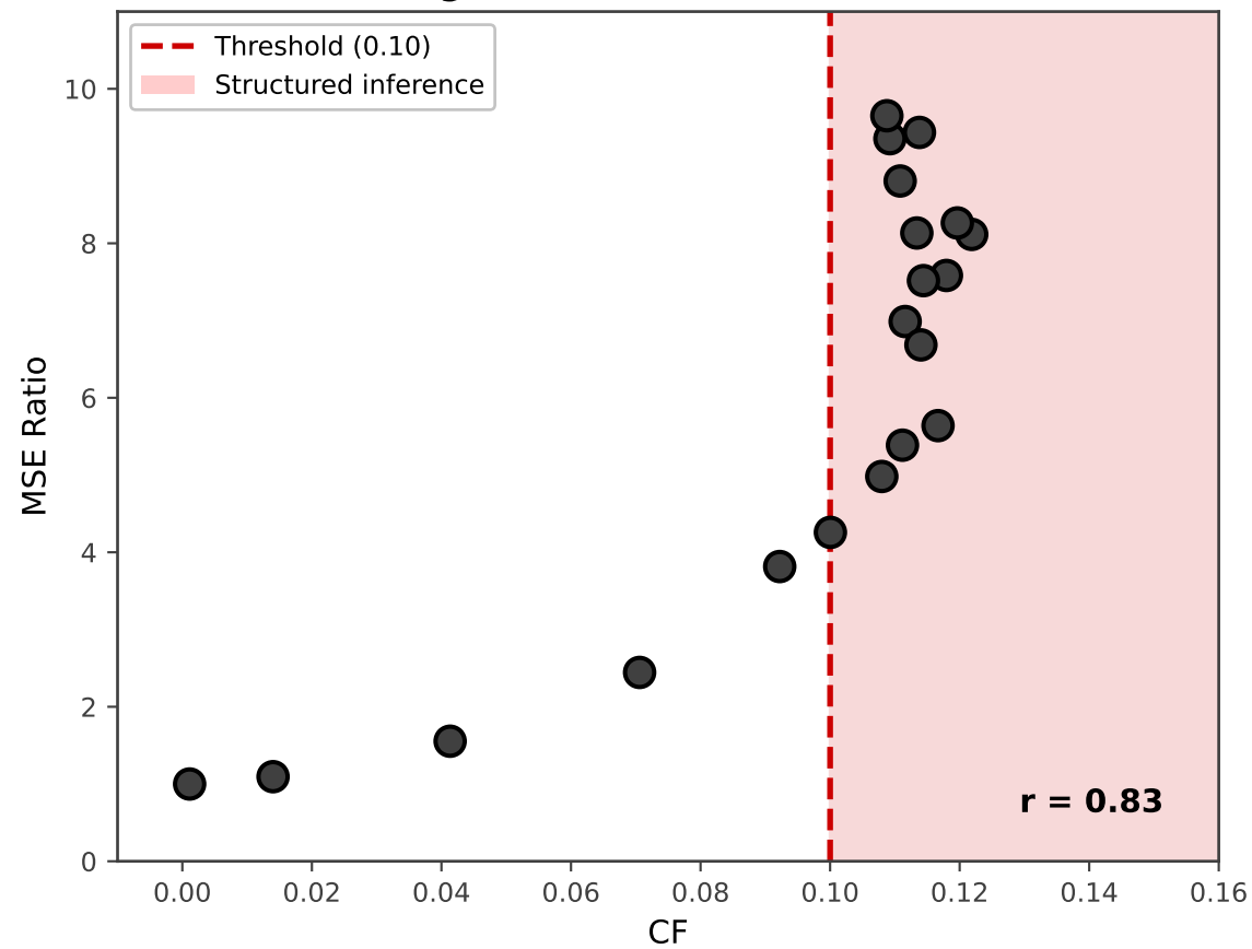
(A) SVF: High CF -> Use structured inference
