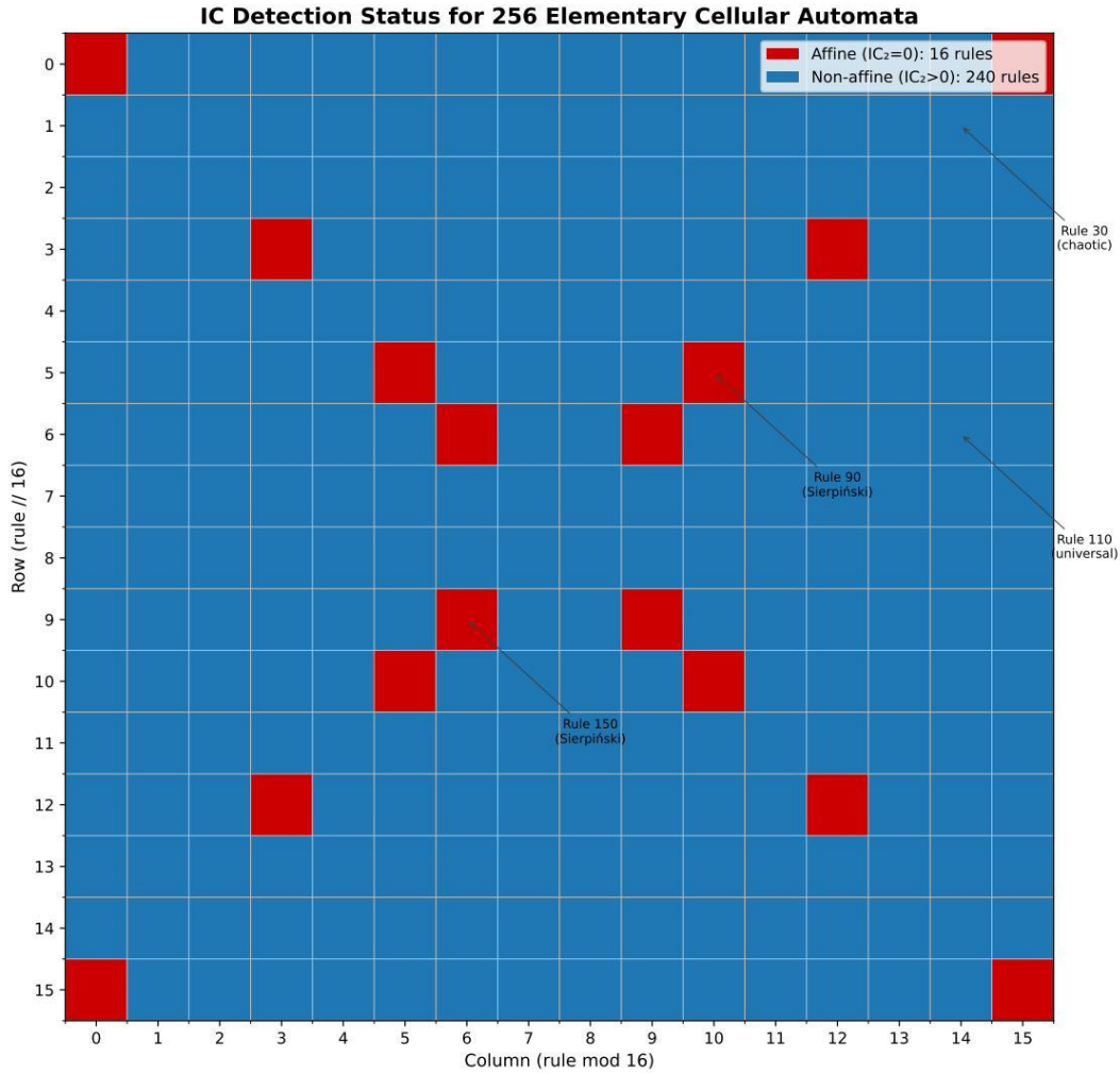
Figure 18: IC detection status for all 256 elementary cellular automata. Each cell represents one ECA rule, arranged in a 16 \times 16 grid (rule number = row \times 16 + column). Red cells: affine rules over \text{GF}(2) where \text{IC}_2 = 0 for all input pairs (16 rules, 6.25%). Blue cells: non-affine rules where \text{IC}_2 > 0 for at least one input pair (240 rules). The 16 affine rules—including Rule 90 and Rule 150 (Sierpiński generators)—exhibit pure synergy invisible to pairwise analysis. Circled rules: notable examples (Rule 30: chaotic; Rule 90/150: Sierpiński; Rule 110: computationally universal). The sparse distribution of affine rules (measure zero in function space) explains why pairwise IC succeeds for most practical models.
