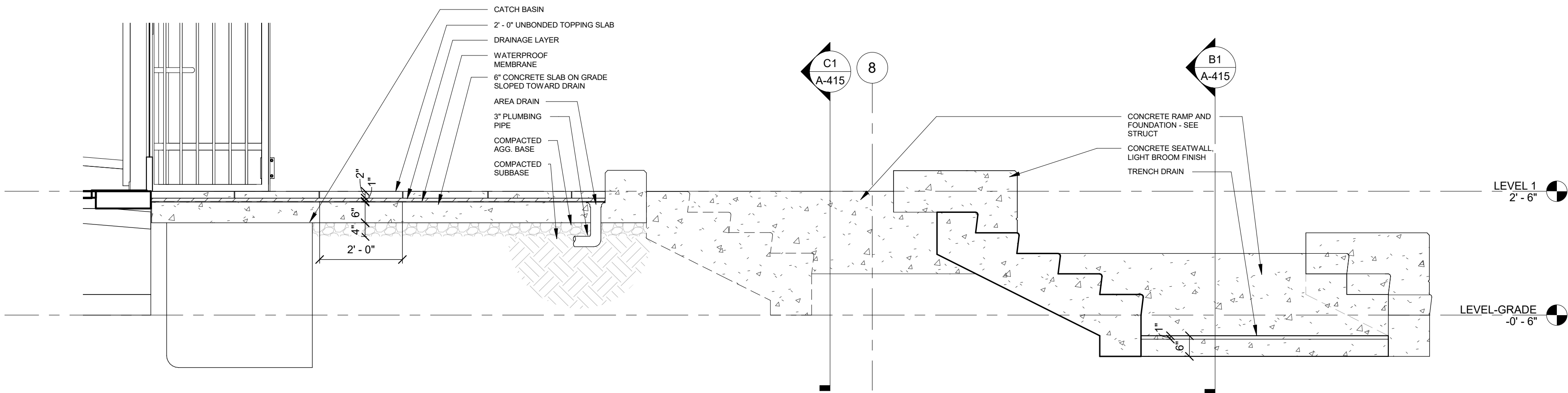
C3 TRANSVERSE SECTION WEST STRAMP 1/2" = 1'-0"
