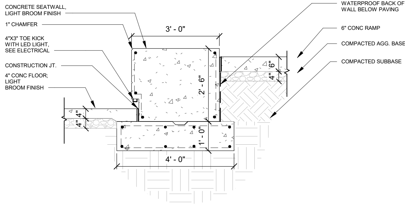
F3 SEATWALL DETAIL 1/2" = 1'-0"
