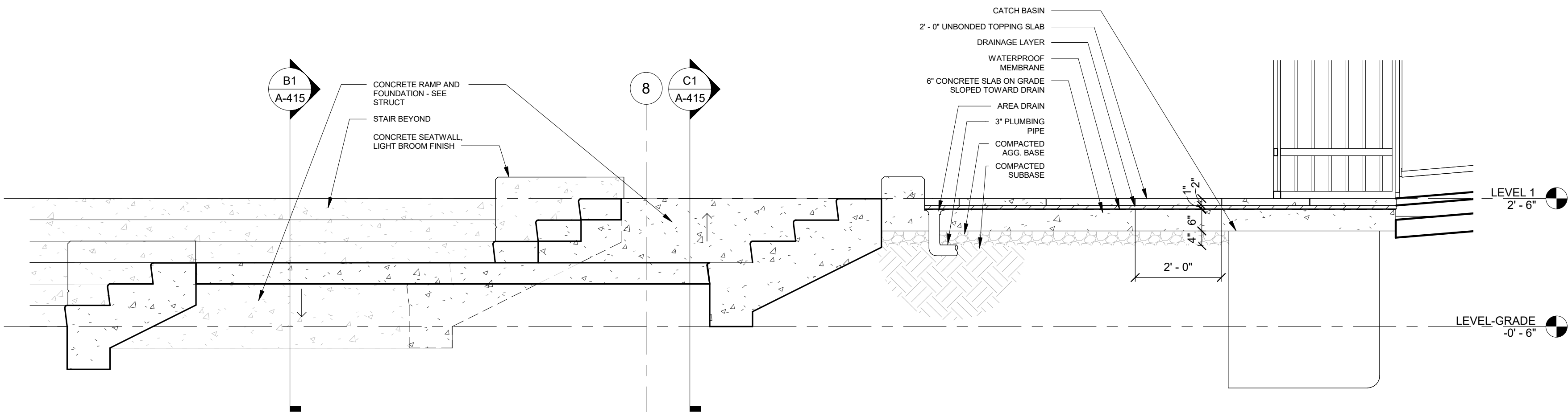
A3 TRANSVERSE SECTION EAST STRAMP 1/2" = 1'-0"
