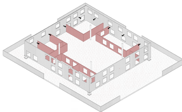
3. Interior CMU walls for first floor added.
