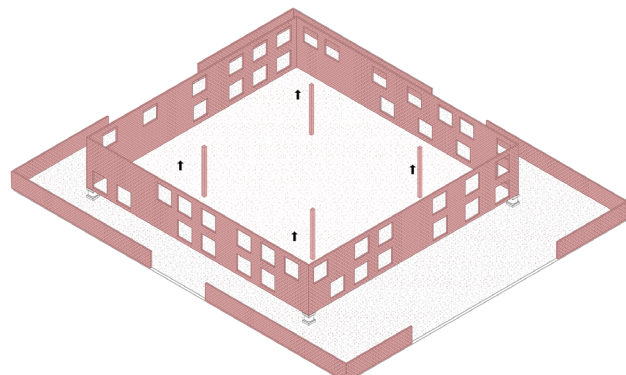
2. Exterior steel-reinforced concrete masonry unit load bearing walls and concrete columns constructed. Concrete masonry walls surrounding building also added.
