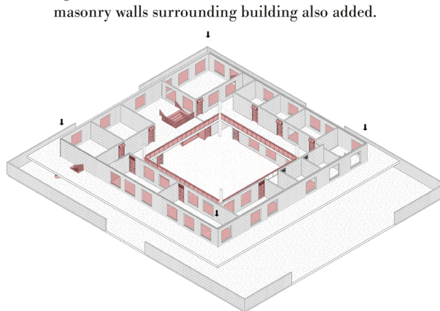
5. Staircases, railings, doors added. Glass for windows if necessary based on site among other specifications.
