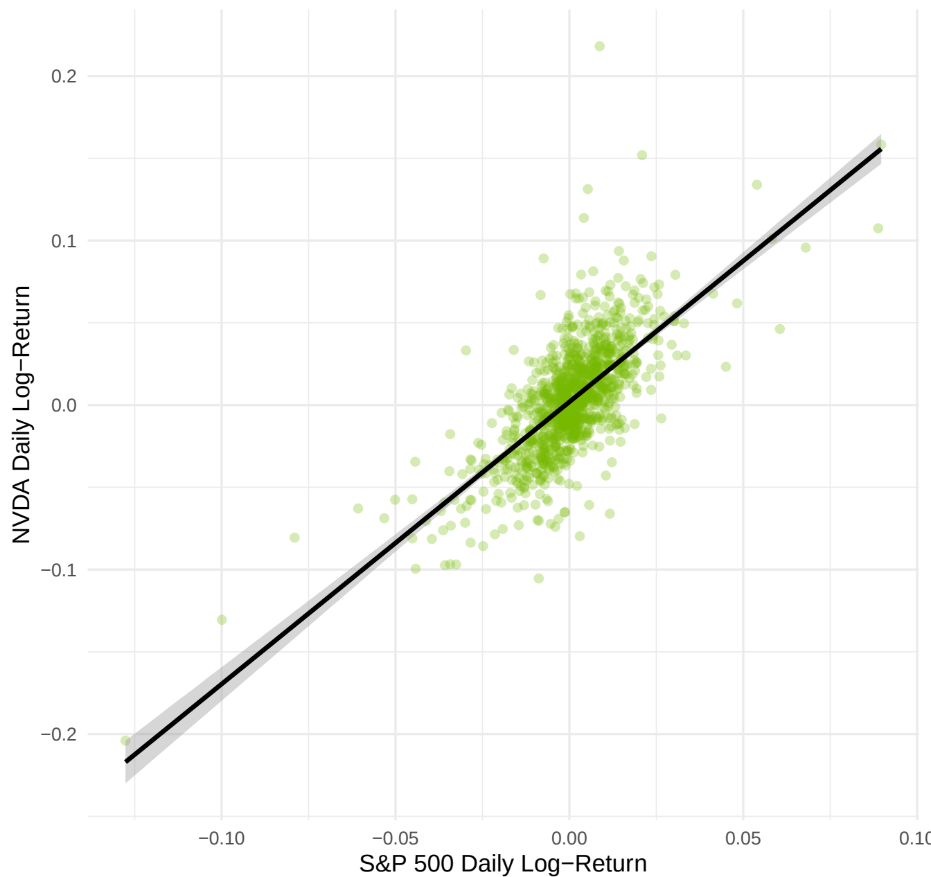
NVDA vs S&P 500 — Market Model ( \beta = 1.71 , R^2 = 0.50 )
