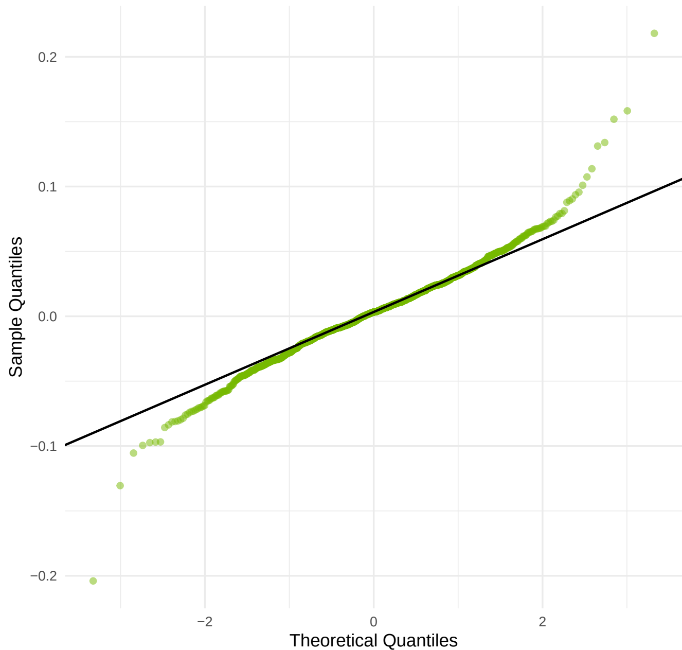
Q-Q Plot — NVDA Daily Log-Returns
