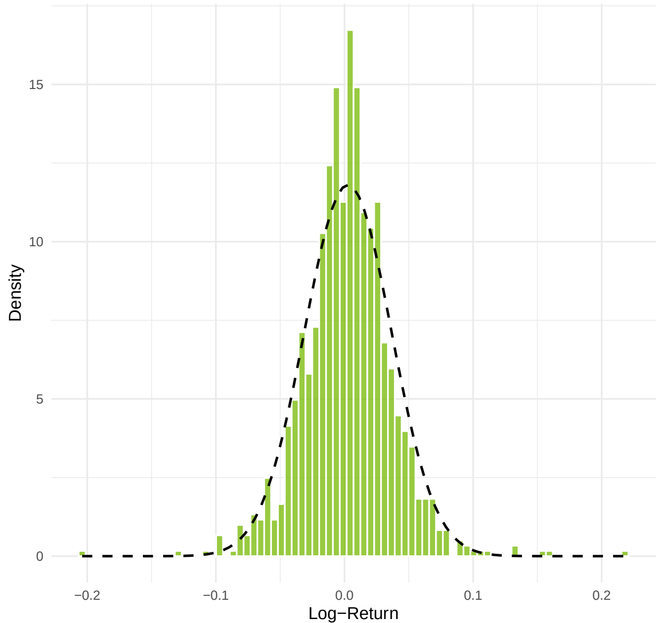
NVDA Daily Log-Returns: Distribution vs Normal
