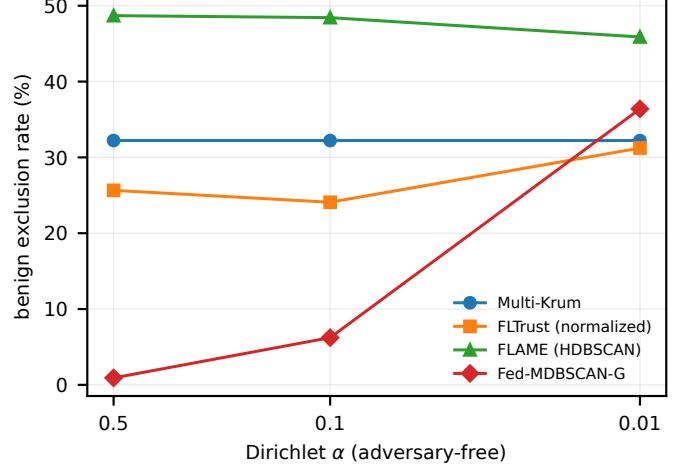
Fig. 2. Adversary-free exclusion, averaged over available dataset cells. Coverage varies by concentration and method. FLTrust counts zero-weight submissions. The FLAME bound need not be attained in every round; direct sizes appear in Table V.
