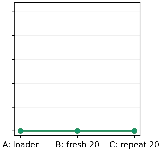
Fashion-MNIST
