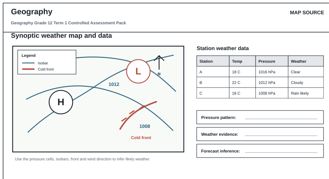
FIGURE 1: Synoptic Weather Map And Data
