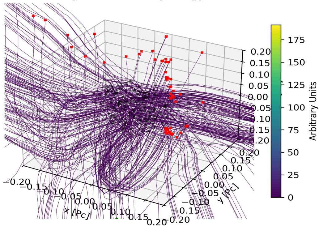
Magnetic field morphology
