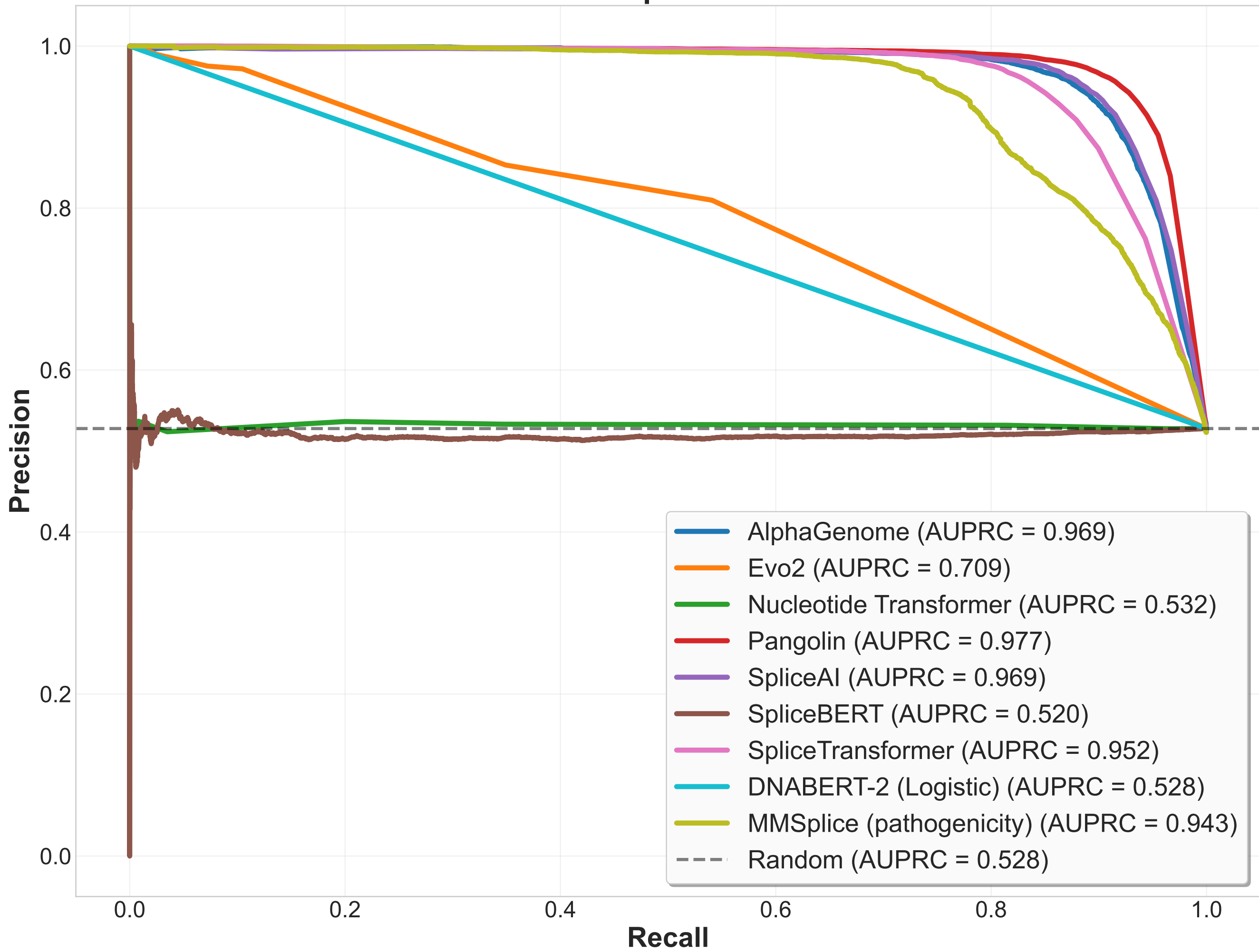
Precision-Recall Curves - SpliceVarDB Human Benchmark
