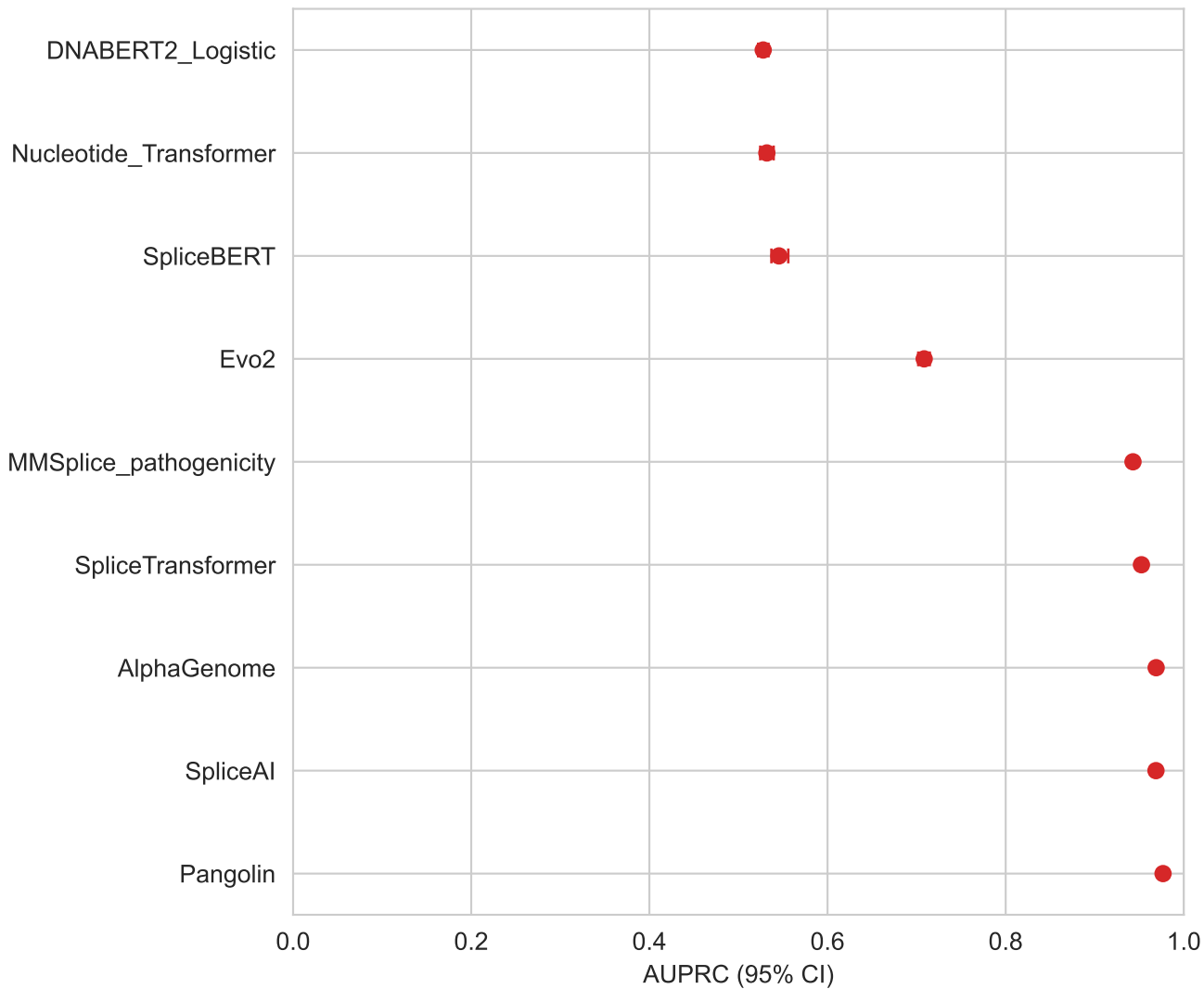
AUPRC with 95% bootstrap CI
