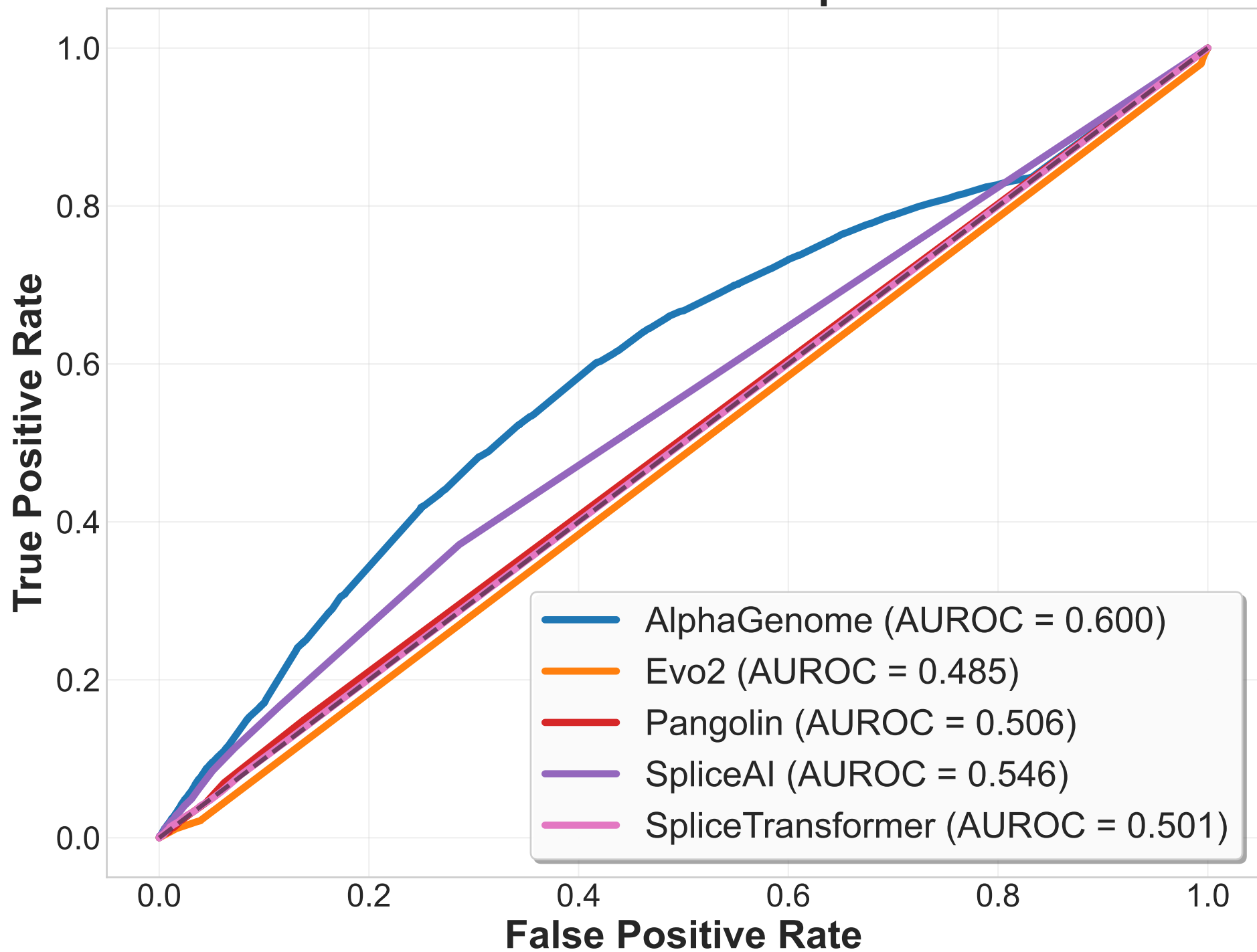
ROC Curves - RatGTEx Cross-Species Benchmark
