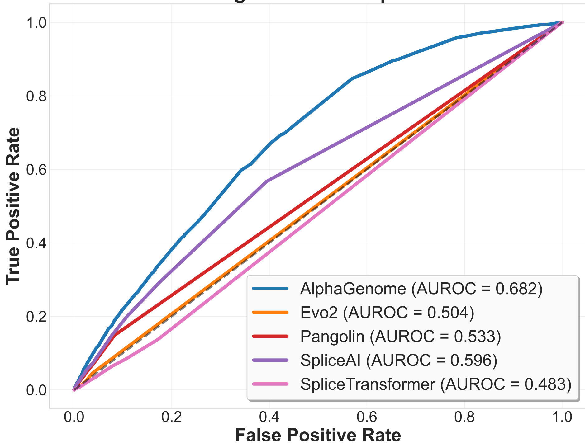
ROC Curves - PigGTEx Cross-Species Benchmark
