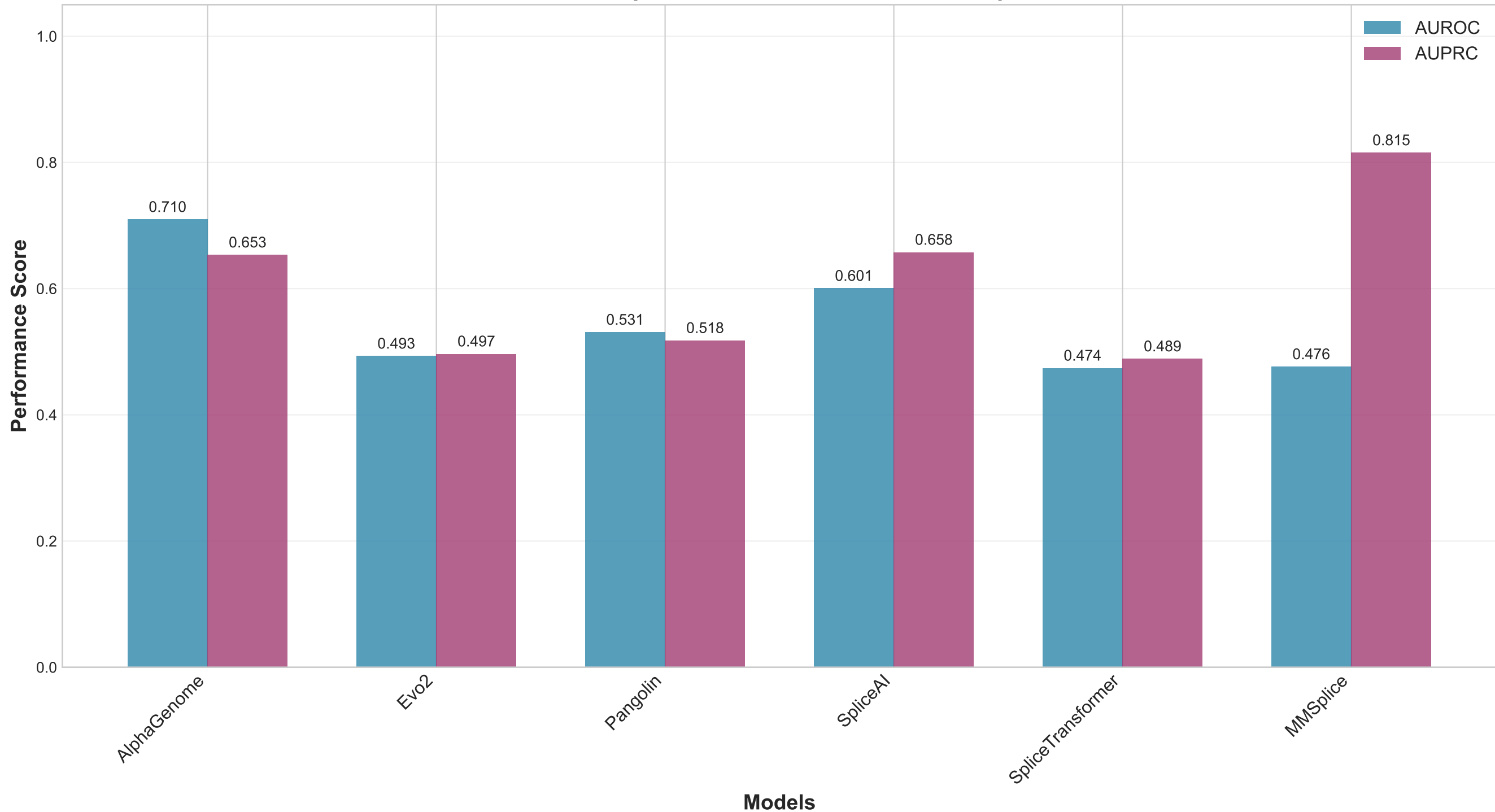
Model Performance Comparison - ChickenGTEx Cross-Species Benchmark
