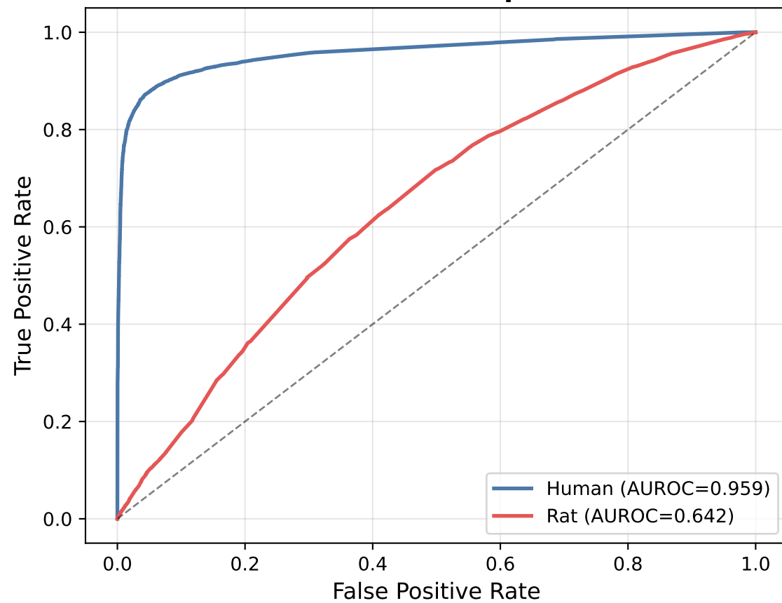
ROC Curves Comparison
