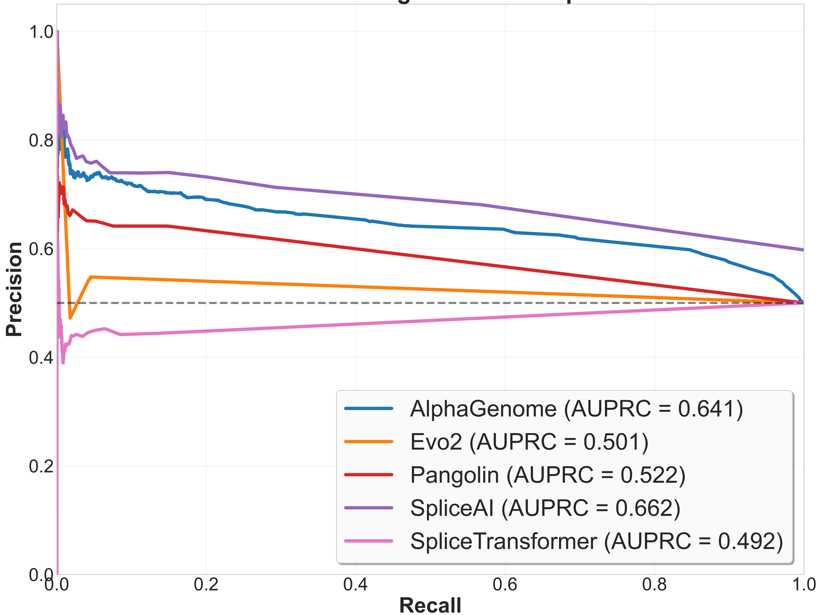
Precision-Recall Curves - PigGTEx Cross-Species Benchmark
