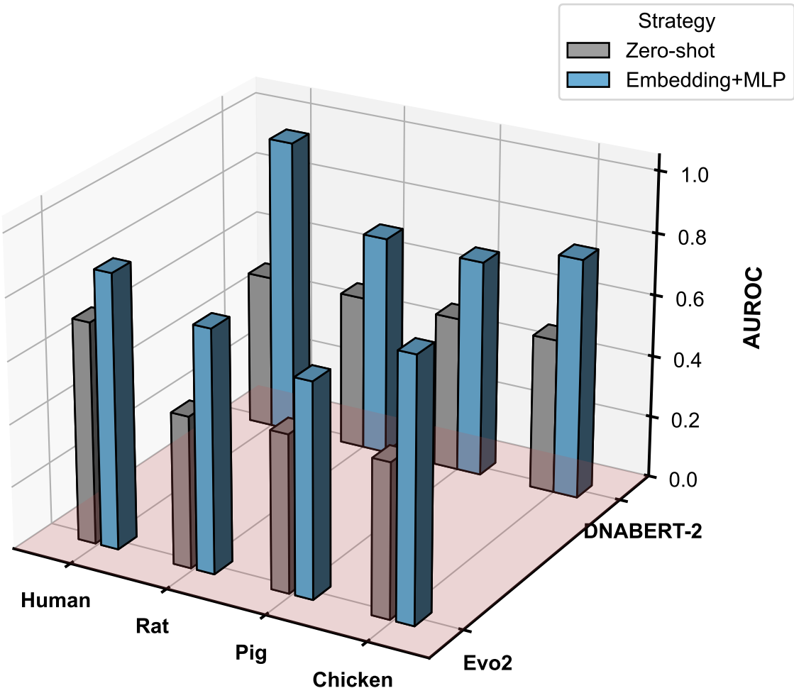
Two-Layer Strategy Comparison (3D) — Front: Evo2, Back: DNABERT-2
