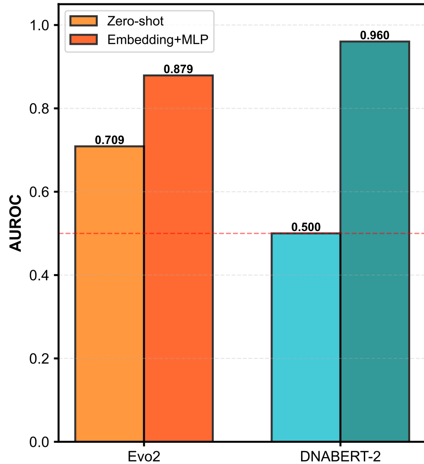
(A) Human (SpliceVarDB)
