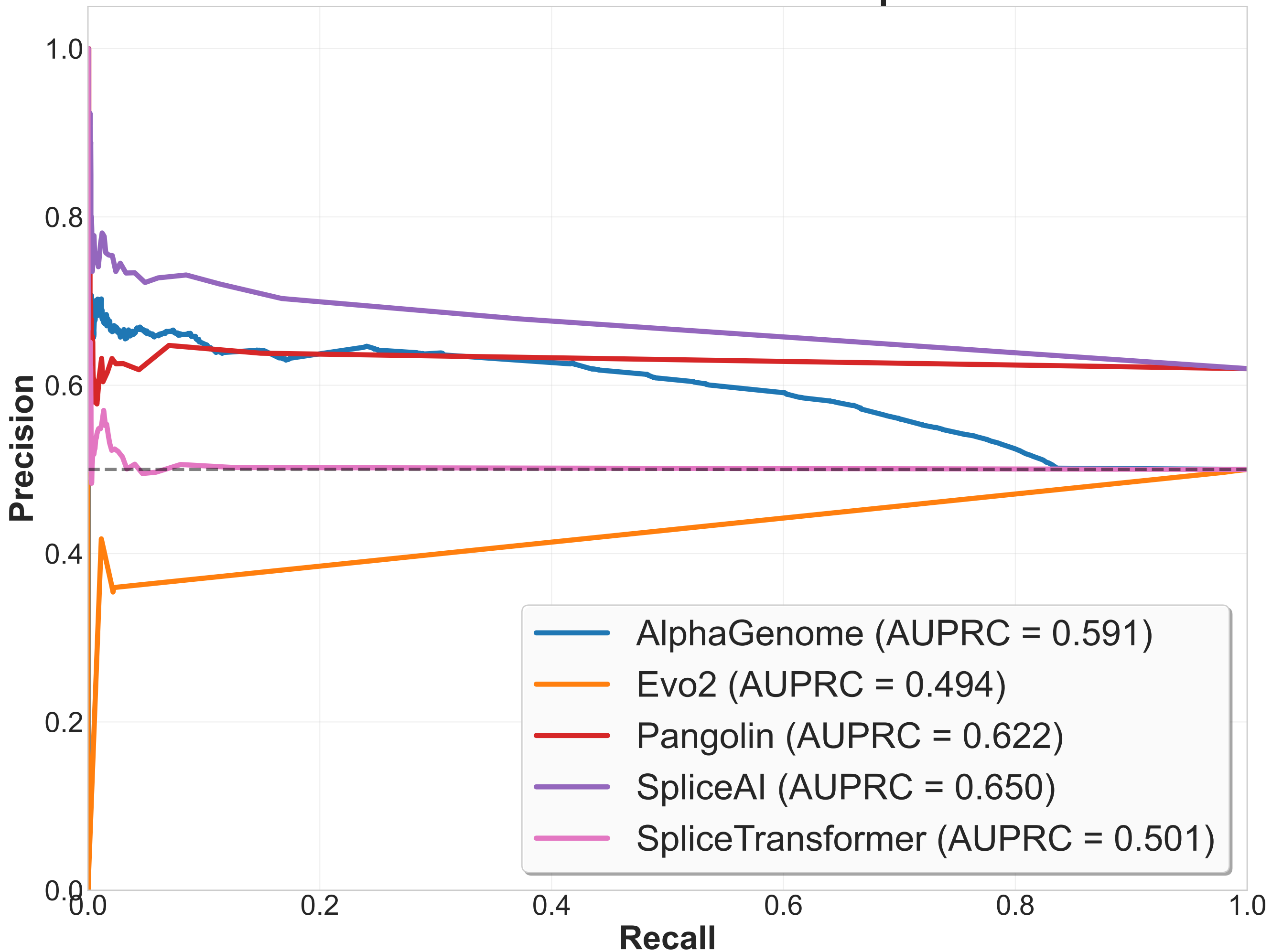
Precision-Recall Curves - RatGTEx Cross-Species Benchmark
