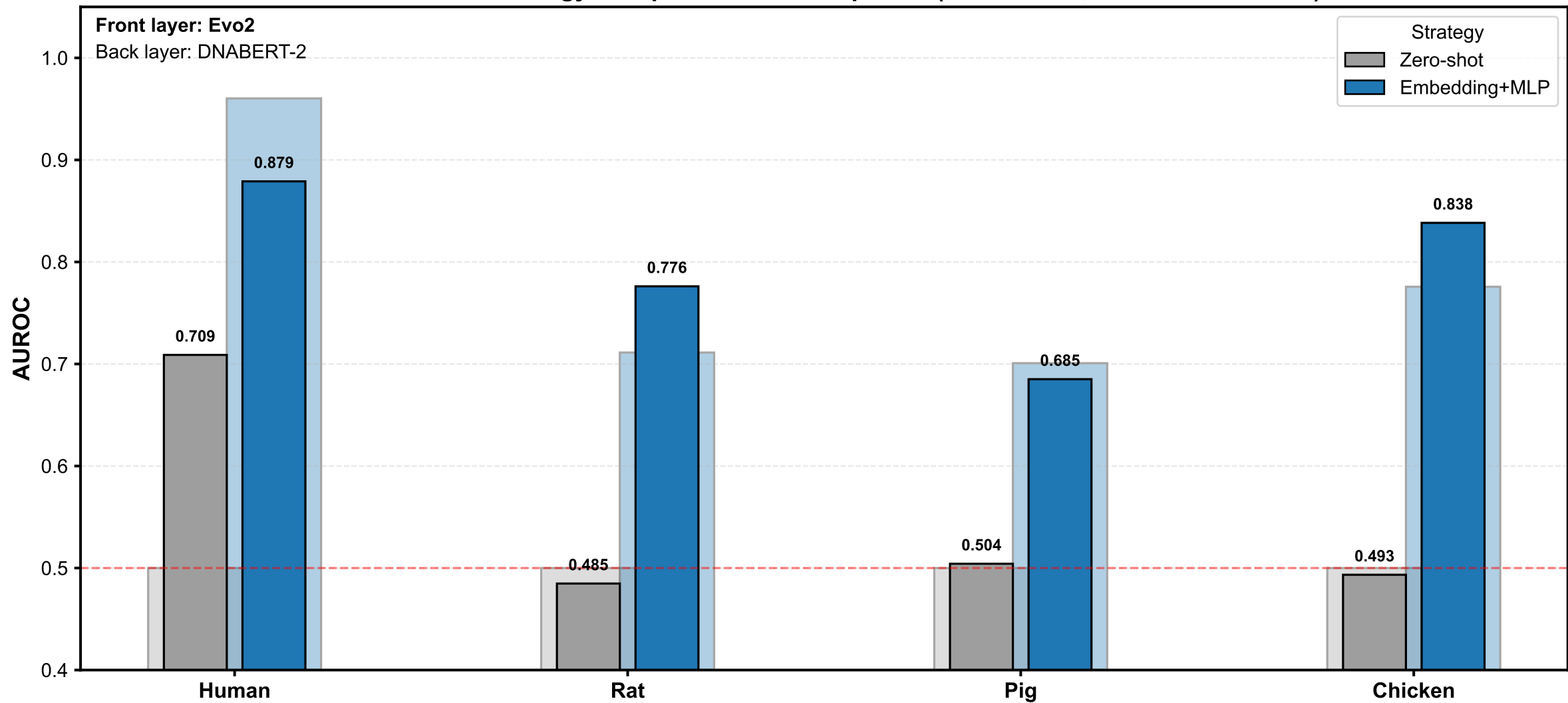
Within-Model Strategy Comparison across Species (Front: Evo2; Back: DNABERT-2)
