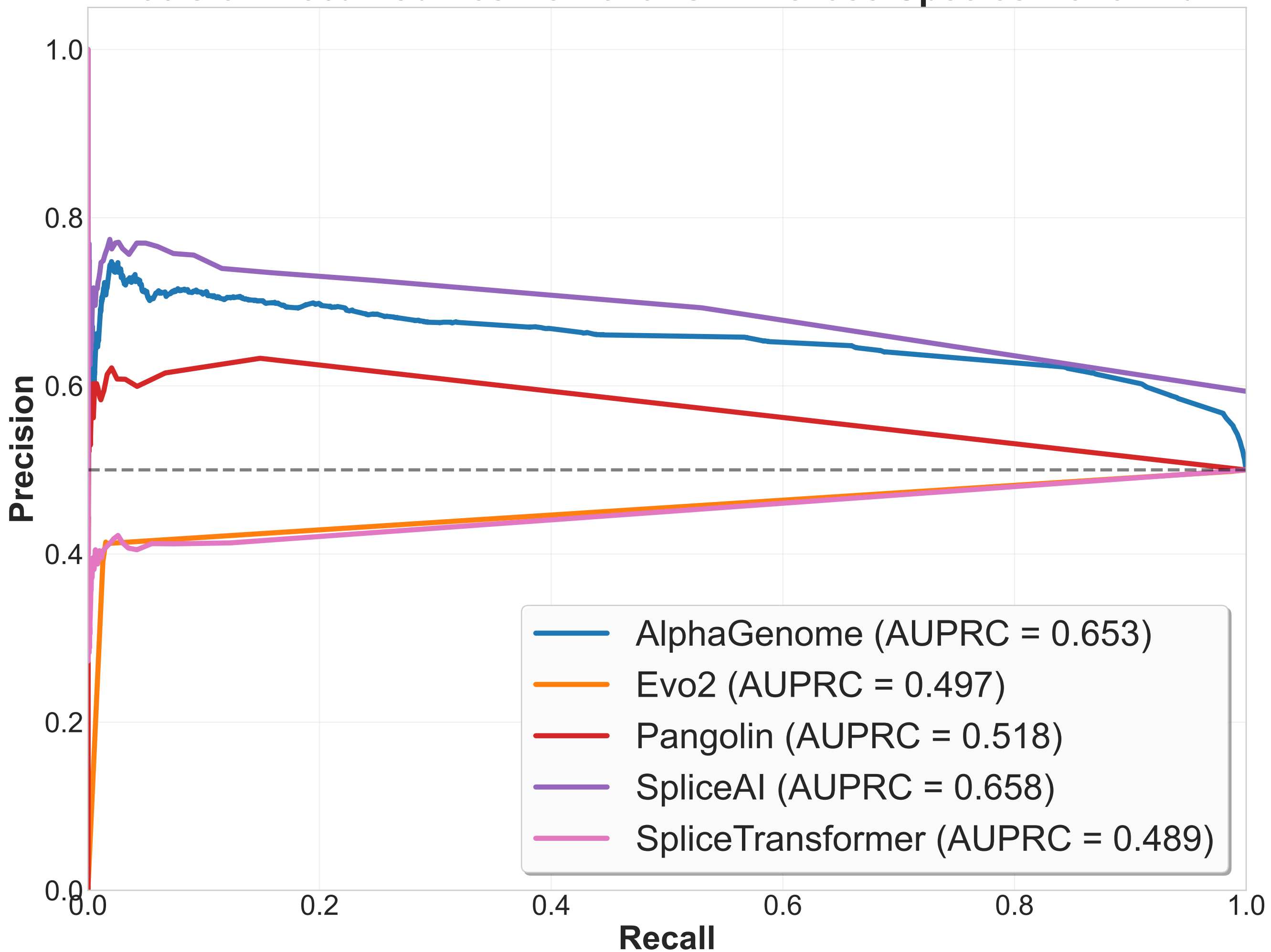
Precision-Recall Curves - ChickenGTEx Cross-Species Benchmark
