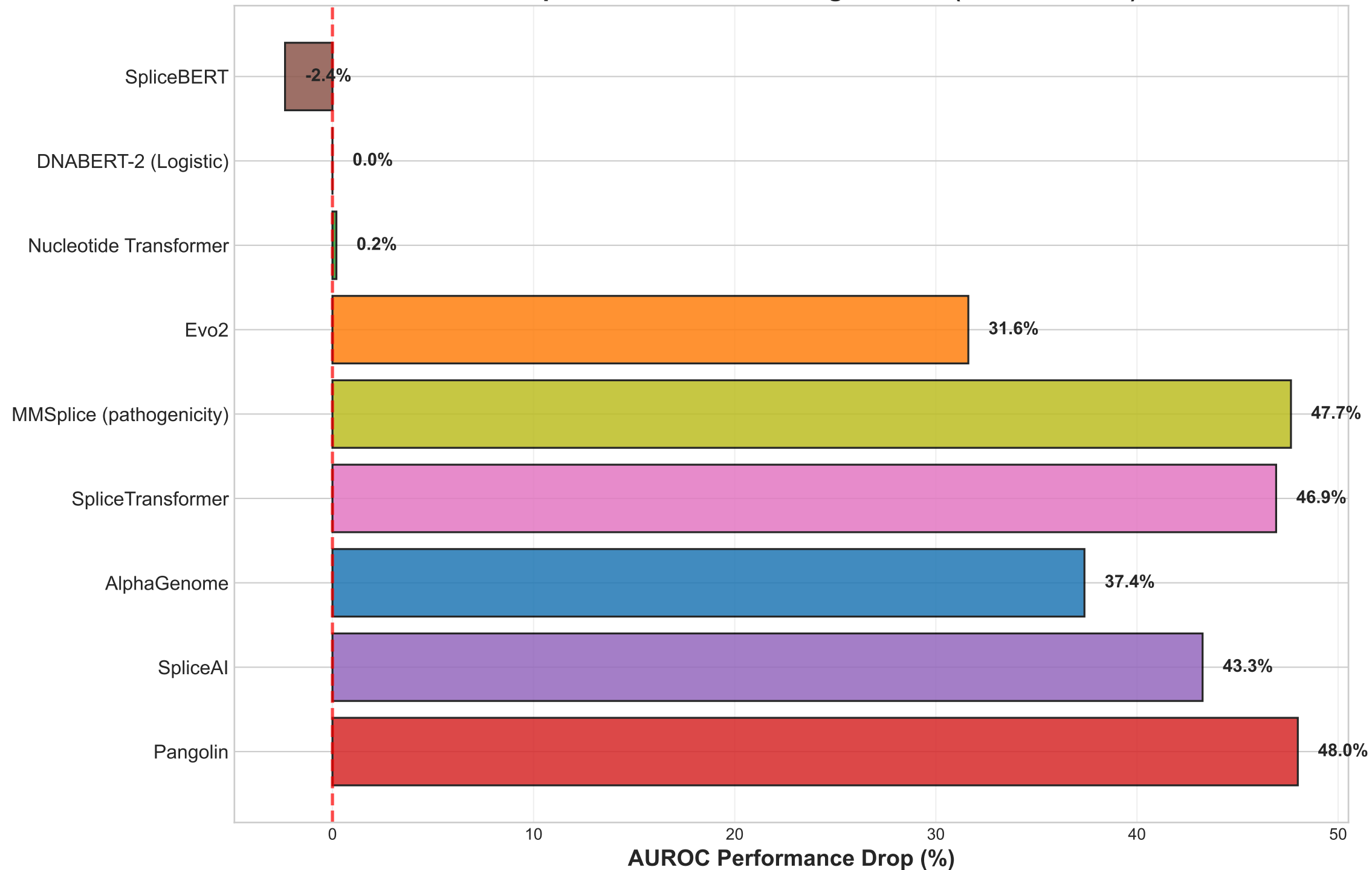
Cross-Species Performance Degradation (Human → Rat)
