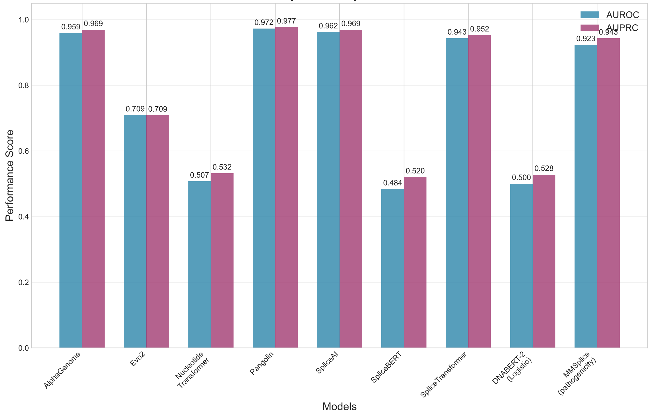
Model Performance Comparison - SpliceVarDB Human Benchmark
