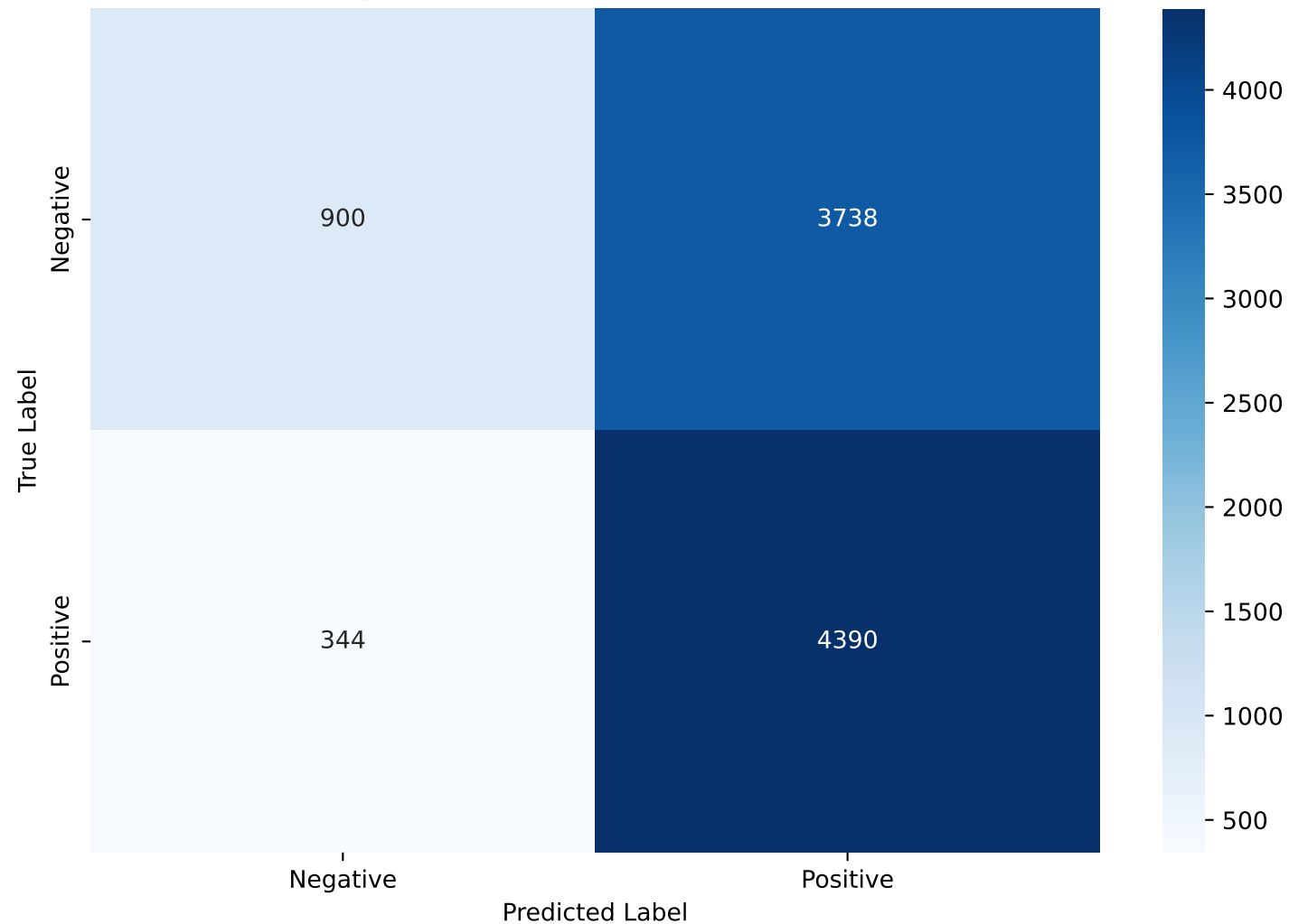
Rat (ratGTE x ) Confusion Matrix AlphaGenome, threshold=0.000732
