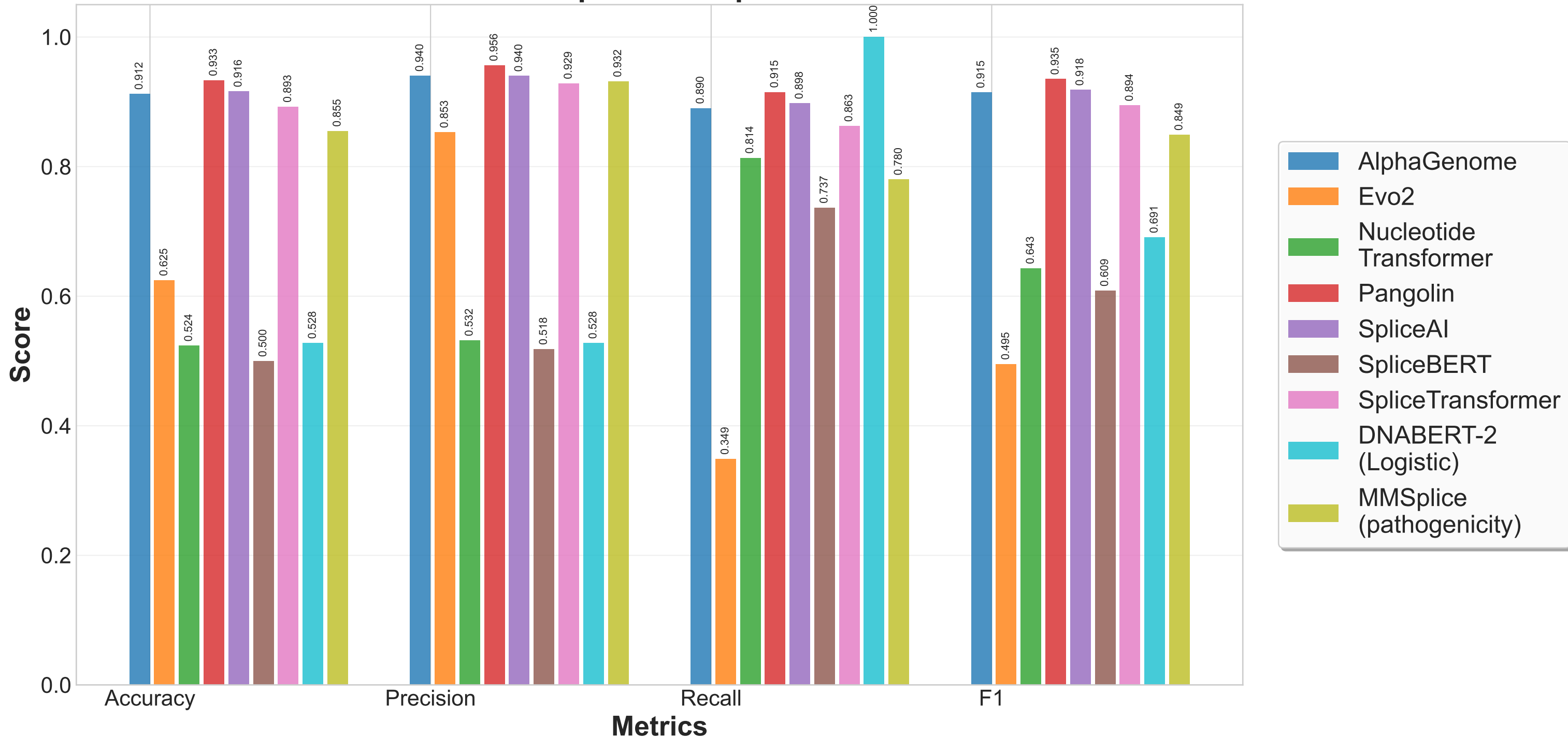
Threshold-Based Metrics Comparison - SpliceVarDB Human Benchmark
