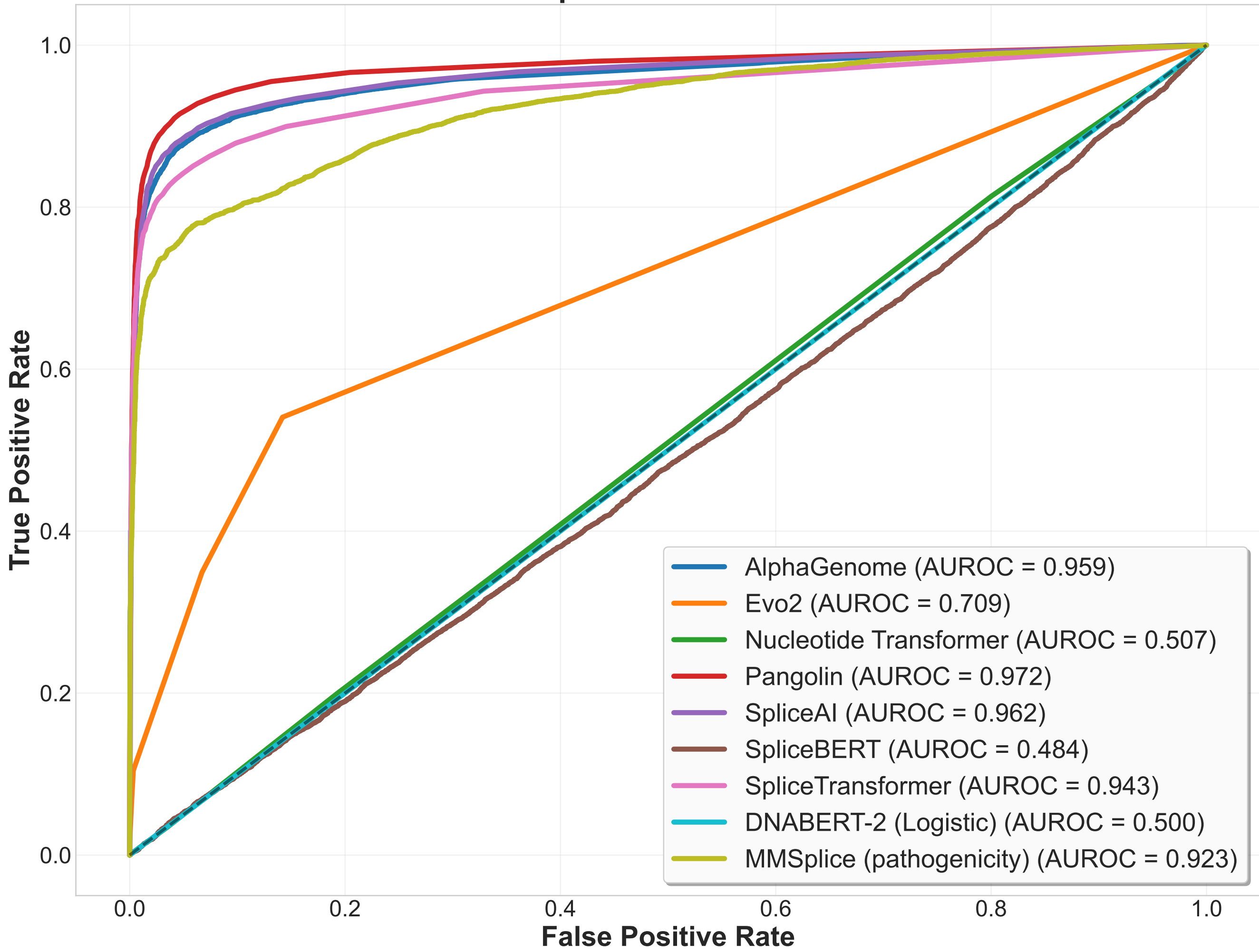
ROC Curves - SpliceVarDB Human Benchmark
