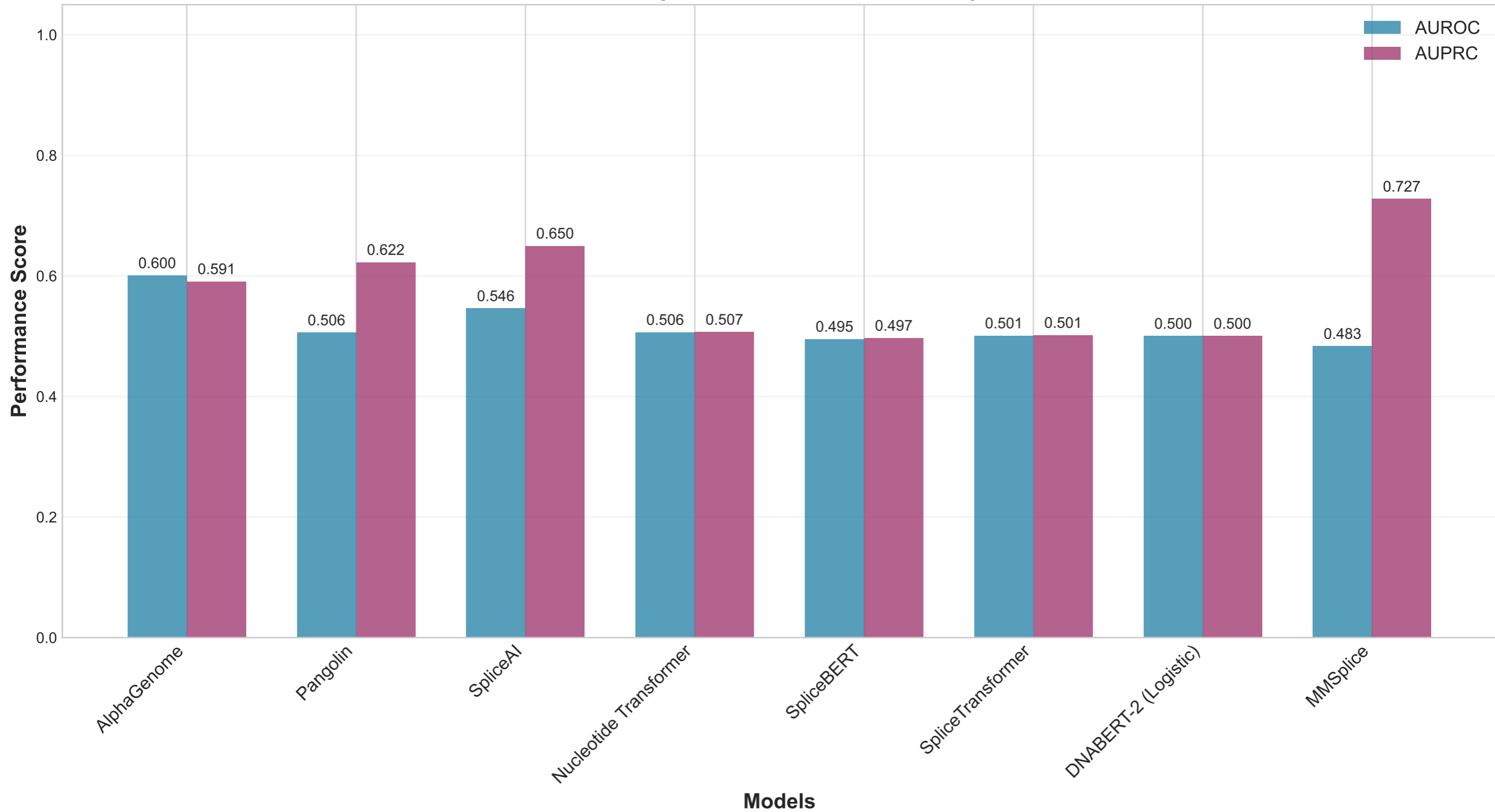
Model Performance Comparison - RatGTEx Cross-Species Benchmark
