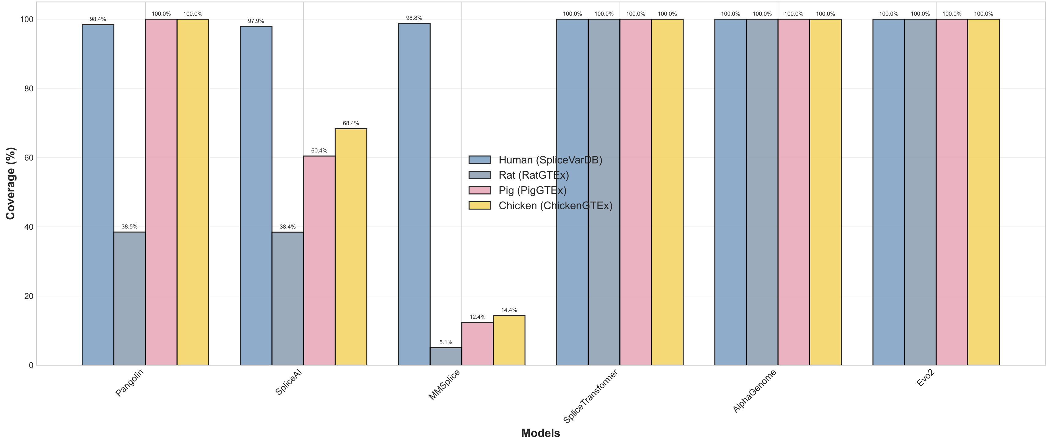
Cross-Species Coverage Comparison
