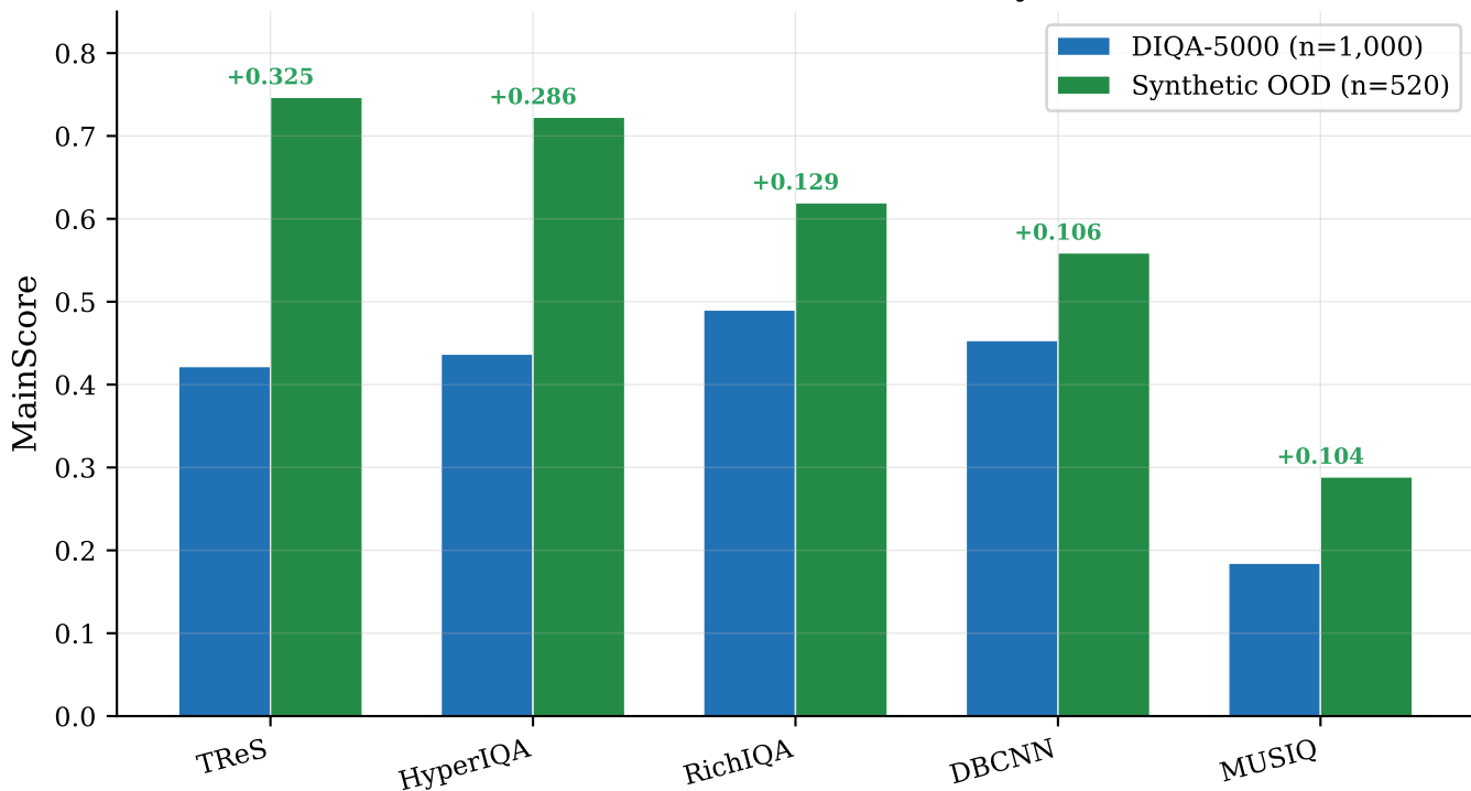
NR-IQA Performance: DIQA-5000 vs Synthetic OOD
