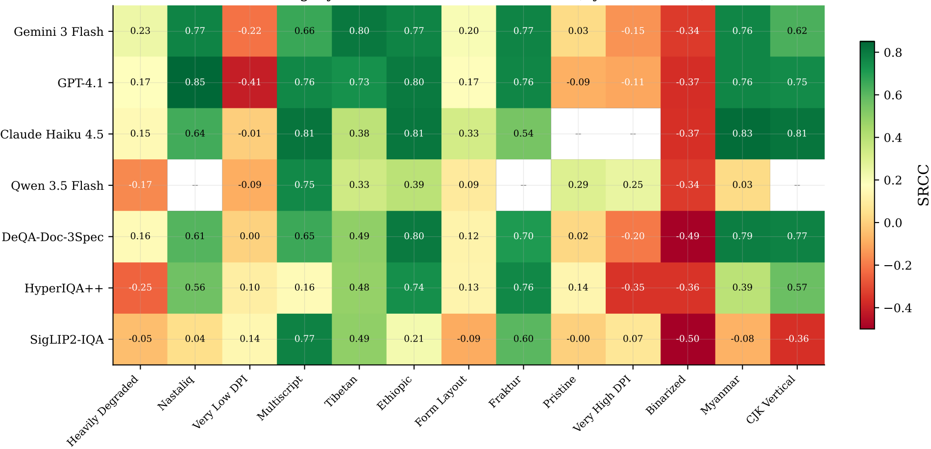
Per-Category Overall SRCC Across Models (Synthetic OOD)
