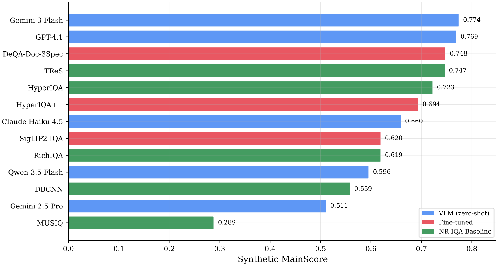
Fine-Tuned Models vs VLMs vs NR-IQA Baselines (Synthetic Dataset)
