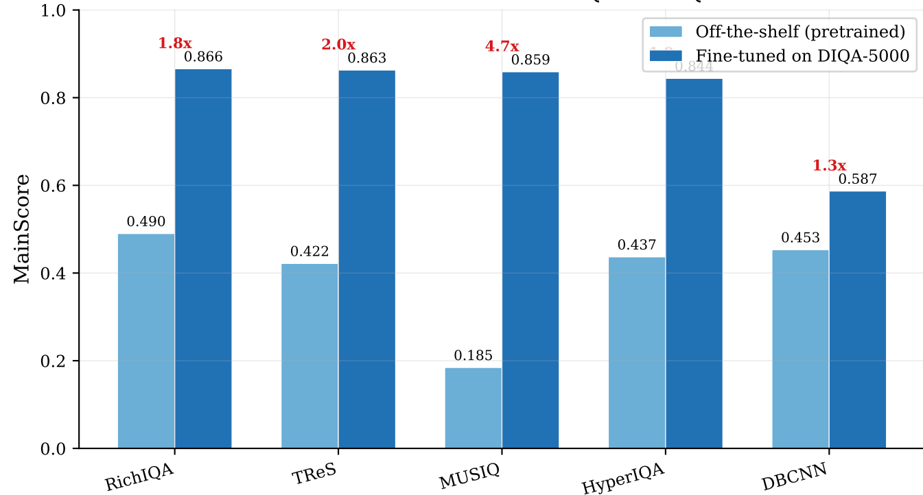
Off-the-Shelf vs Fine-Tuned NR-IQA on DIQA-5000
