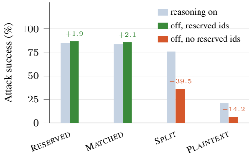
(b) Reasoning block on and suppressed
