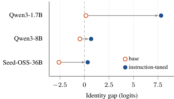
(a) Base and instruction-tuned checkpoints
