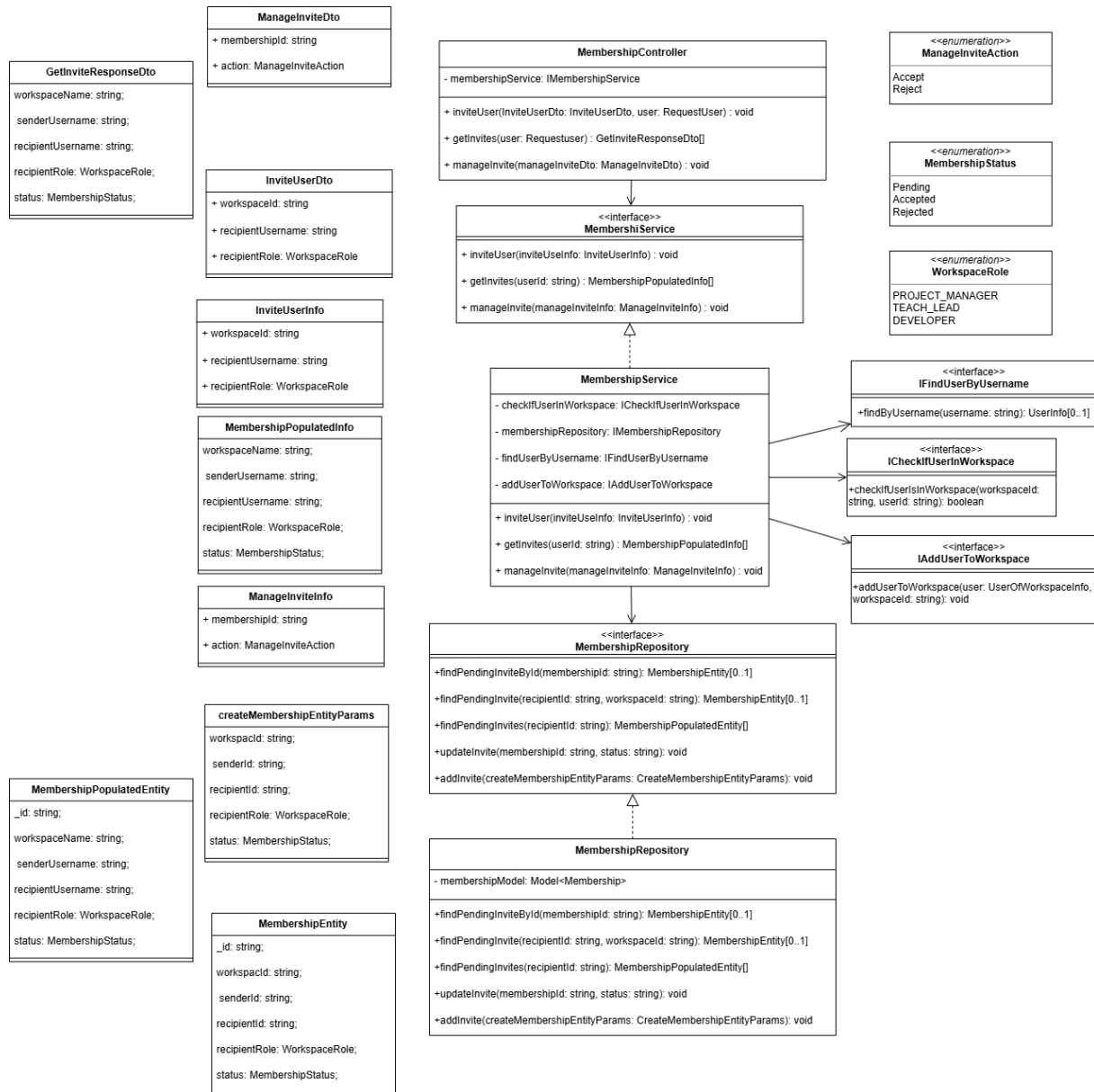
Figura 11: UML Modulo Membership
