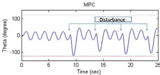
Figure 6. Arm angle
