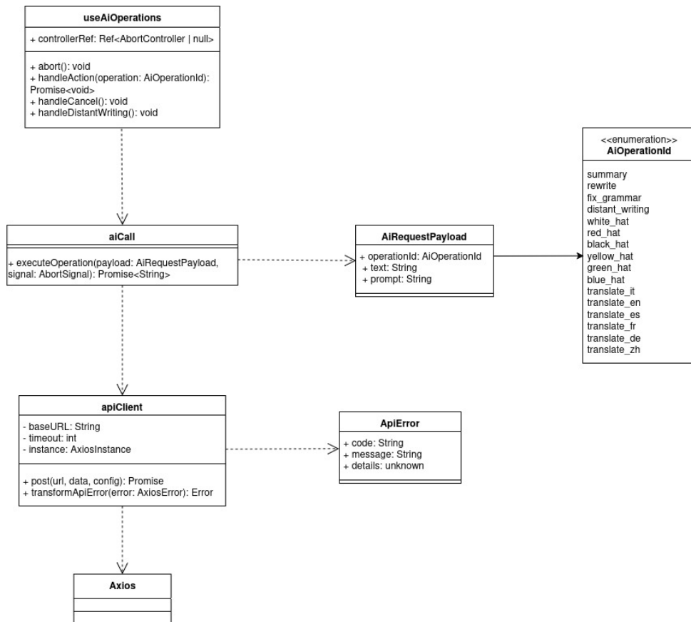
Figura 8: UML del pattern Facade
