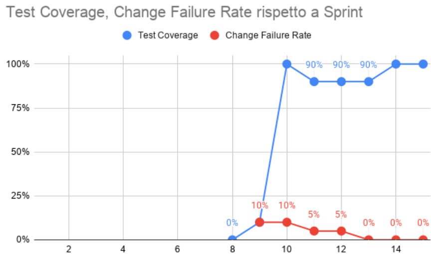
Figura 17: Test Coverage, Change Failure Rate
