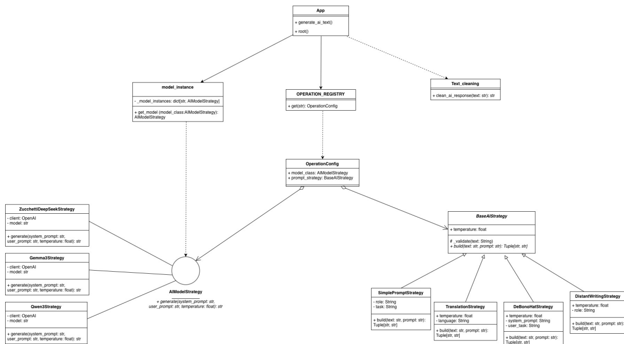
Figura 2: Diagramma UML Backend: layered architecture e strategy pattern
