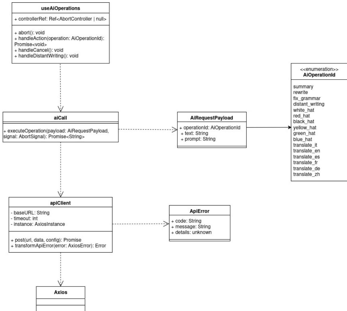
Figura 2: UML del pattern Facade
