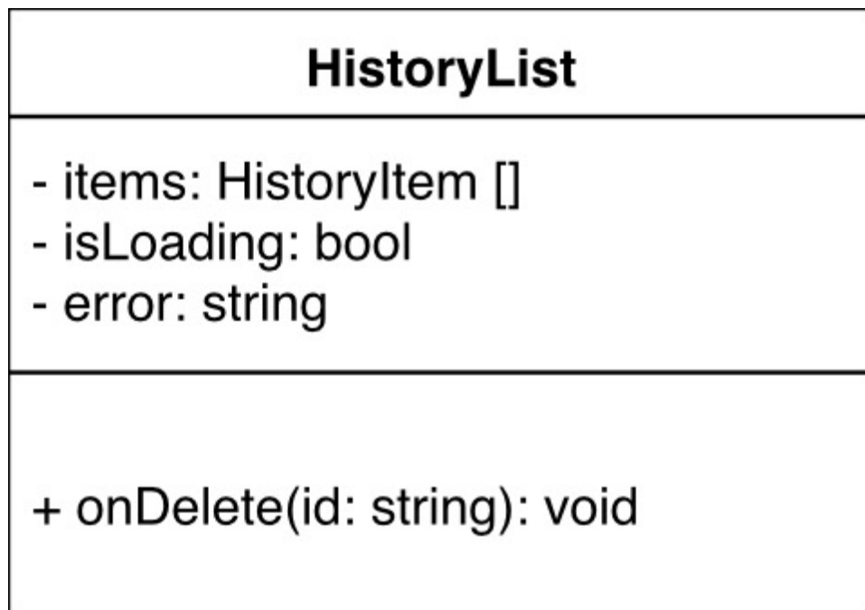
Figura 7: UML HistoryList
