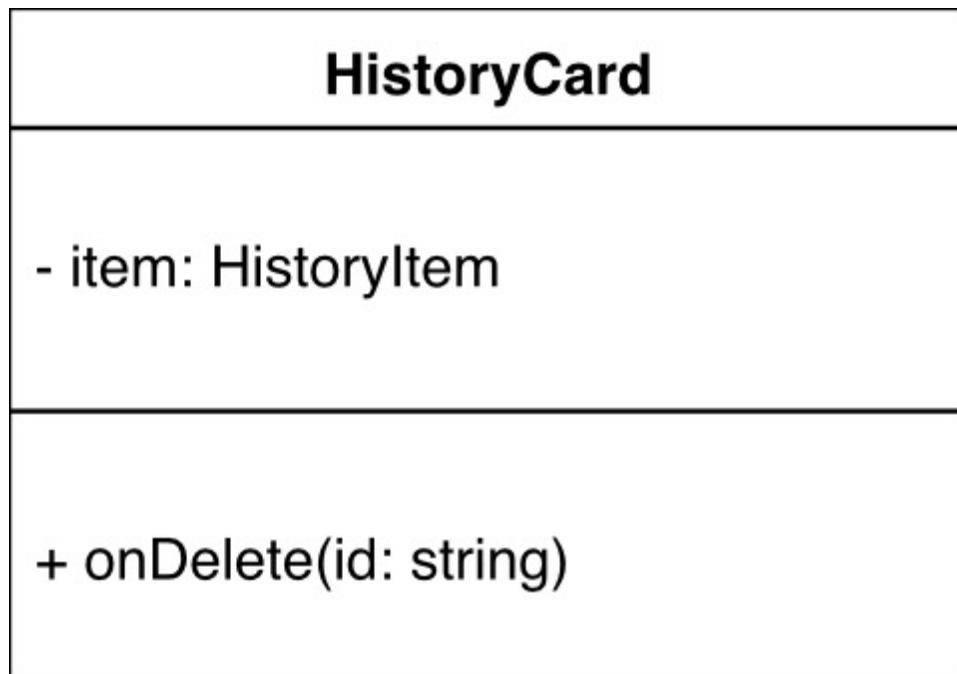
Figura 8: UML HistoryCard
