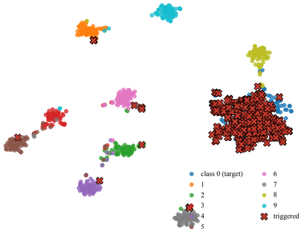
Feature space (t-SNE)
