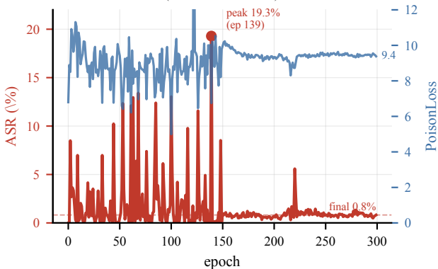
KST on GTSRB ( \epsilon 48 ): briefly learned, then rejected (victim BA \approx 100 )
