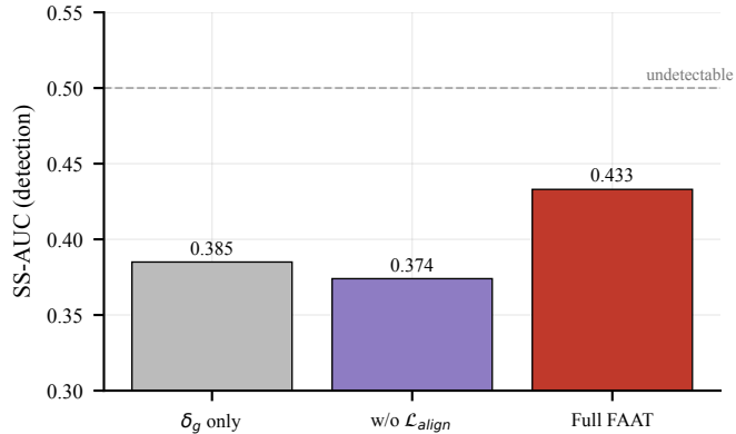
(b) Defense evasion (SS)
