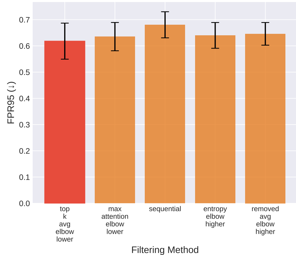
FPR95 (↓) by Filtering Method
