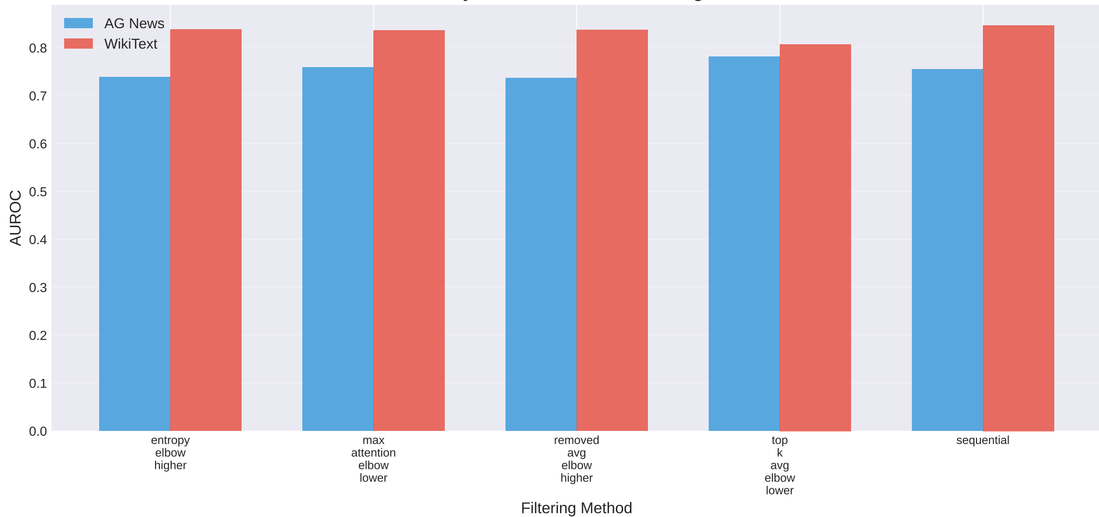
AUROC by OOD Dataset and Filtering Method
