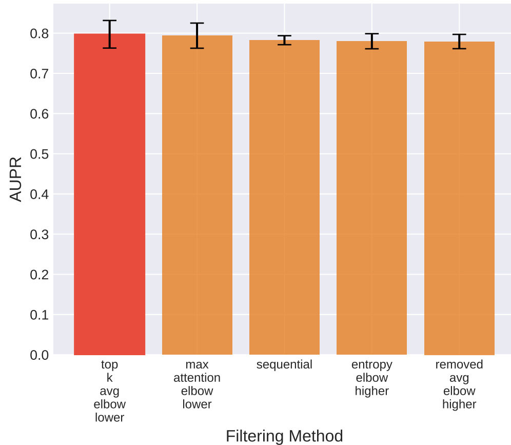
AUPR by Filtering Method
