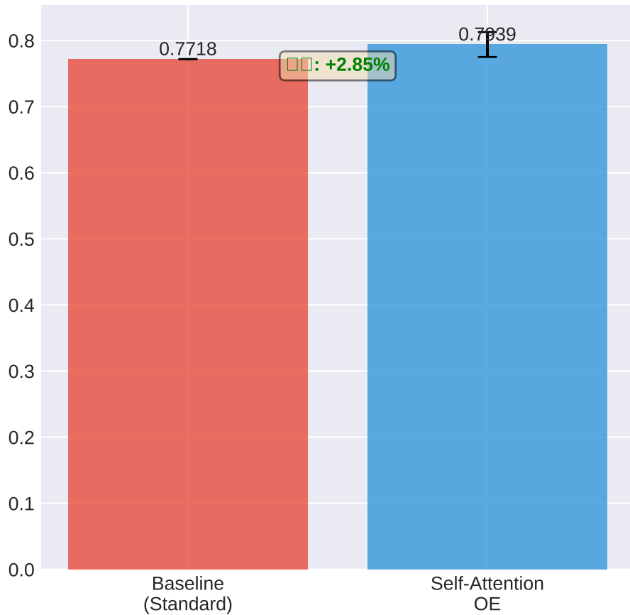
AUROC Comparison
