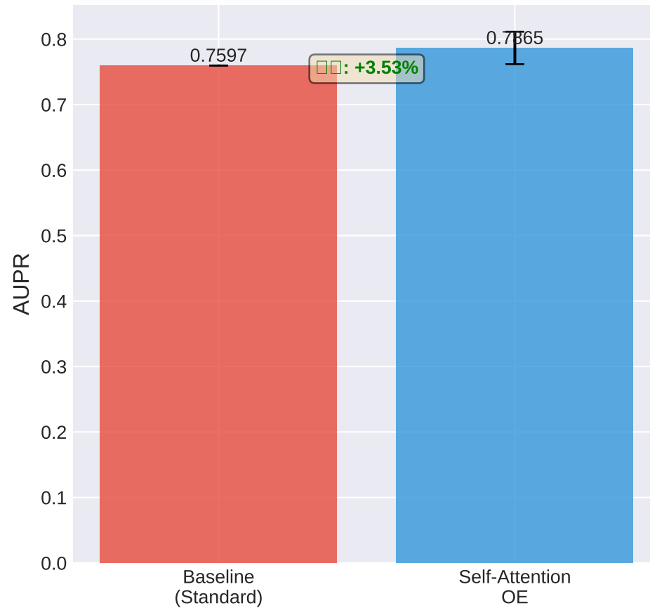
AUPR Comparison
