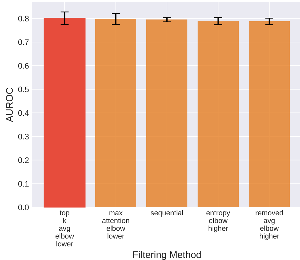
AUROC by Filtering Method
