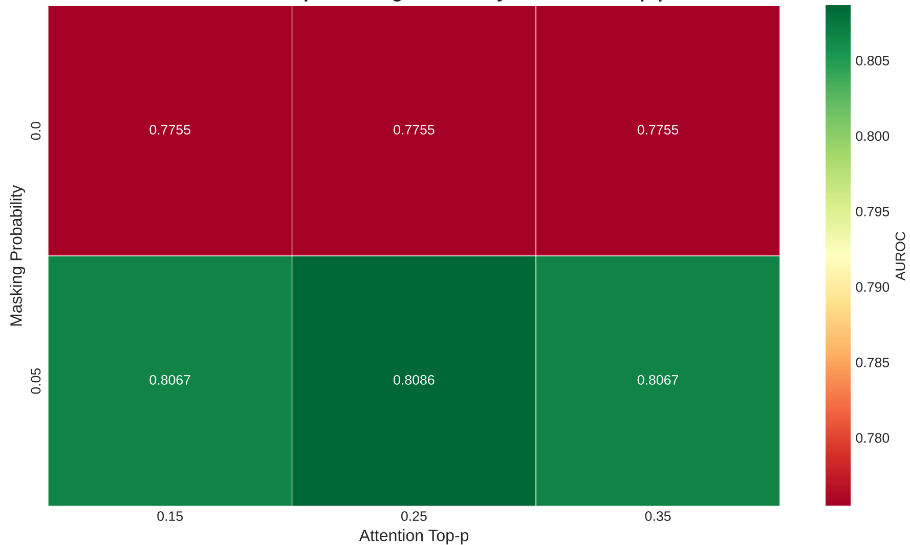
AUROC Heatmap: Masking Probability × Attention Top-p
