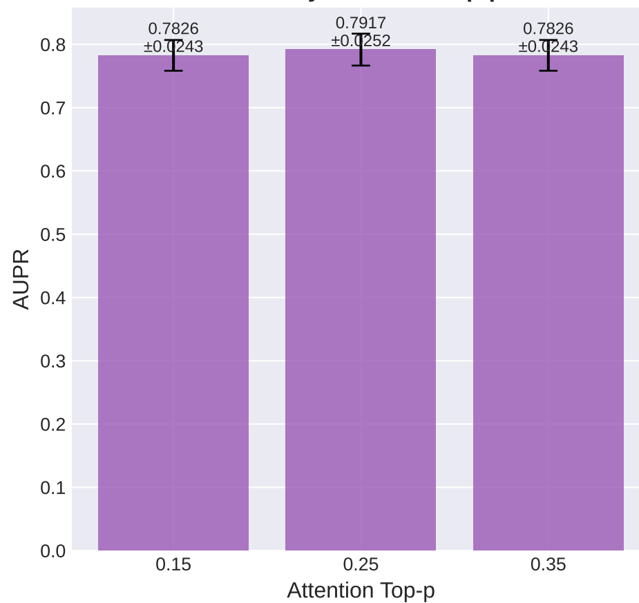
AUPR by Attention Top-p
