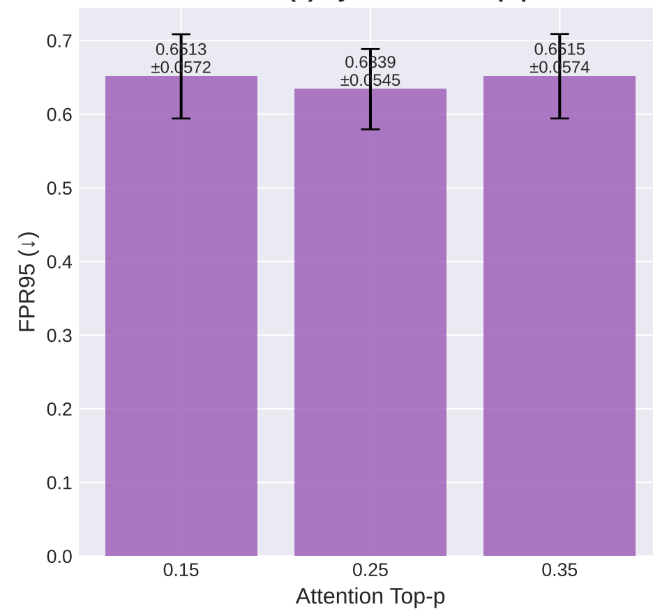
FPR95 (↓) by Attention Top-p
