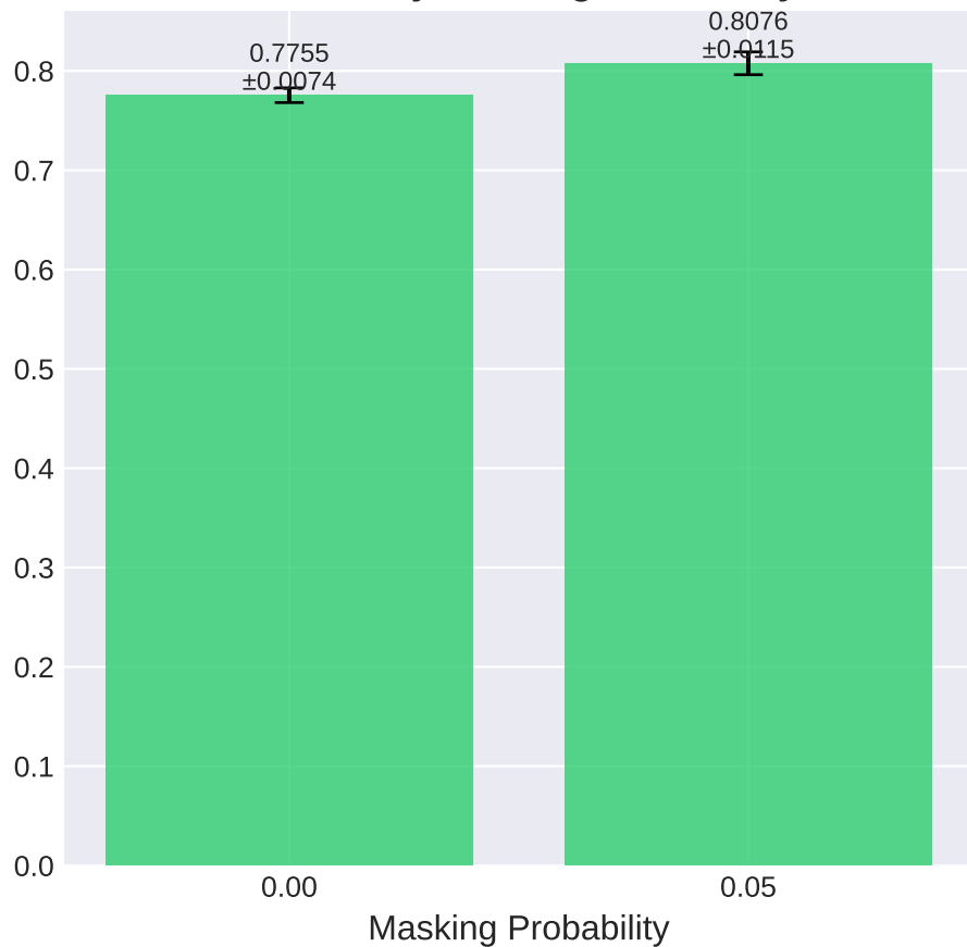
AUROC by Masking Probability
