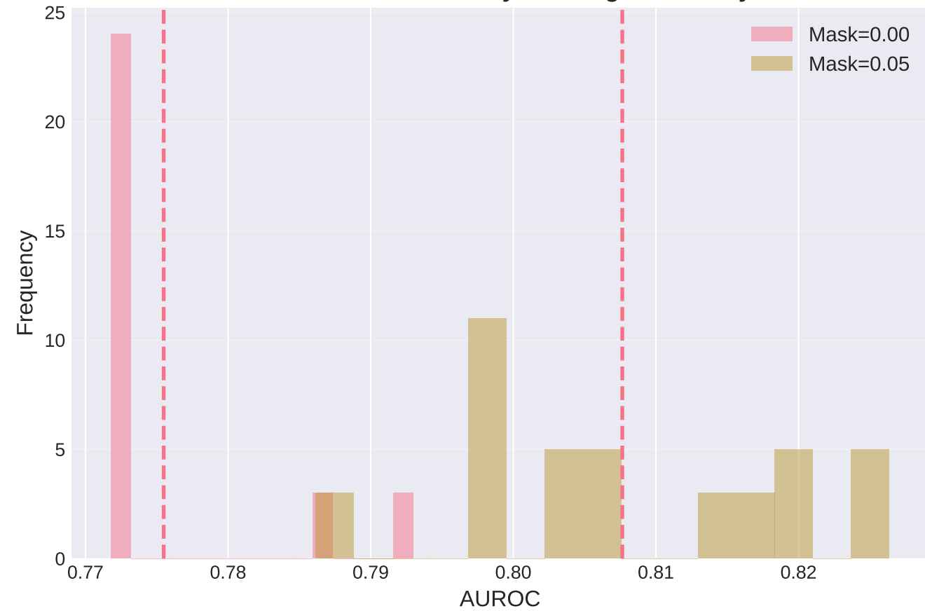
AUROC Distribution by Masking Probability
