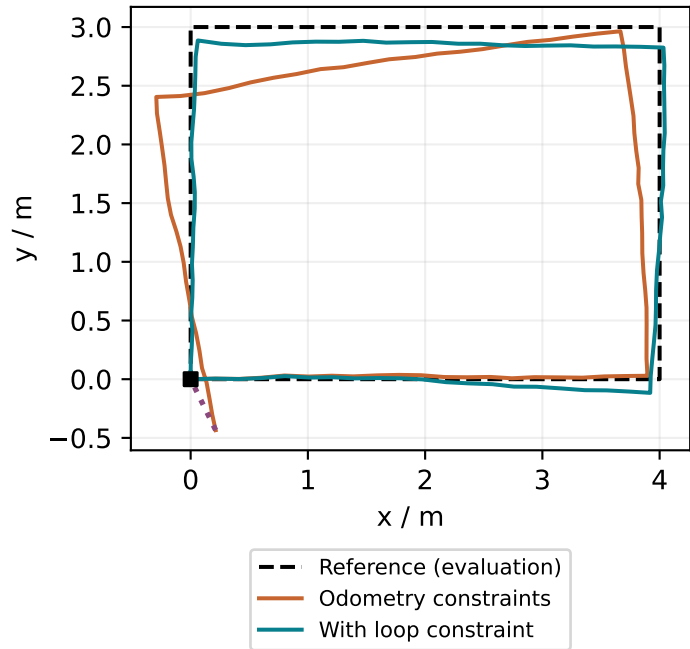
Synthetic square graph, seed 1010
