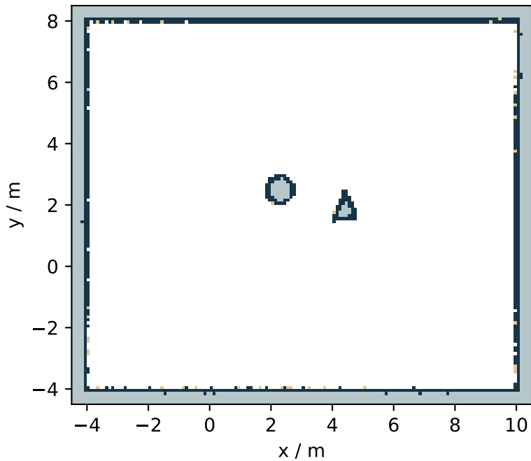
Without loops
