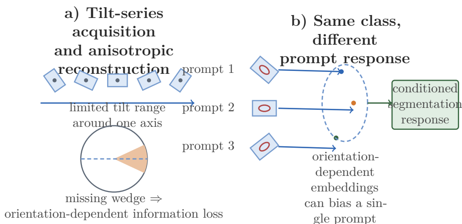
Figure 2.4: Conceptual schematic of why rotational invariance is difficult in cryo-ET. Limited-angle tilt acquisition produces anisotropic reconstructions with a missing wedge, so rotated particles are not observed as simple rigidly rotated copies after reconstruction. When such subtomograms are used as prompts, differences in orientation, reconstruction artifact and local context can lead to different embeddings and different detector responses. This is the conceptual motivation for the prompt-robustness study in EXP4.
