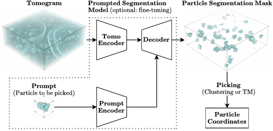
Figure 2.3: Overview of the ProPicker workflow. A prompt encoder extracts features from a reference particle, those features condition the tomogram segmentation model, and the predicted segmentation mask is converted into particle coordinates by a downstream picking step.
