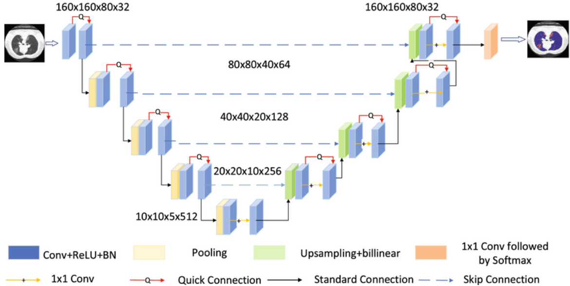
Figure 2.2: Representative 3D U-Net architecture with an encoder-decoder layout, down-sampling through pooling, up-sampling in the decoder, and skip connections that fuse fine and coarse features. In cryo-ET, many localization models keep this same volumetric segmentation pattern while adapting kernels, normalization, supervision targets and post-processing to particle-picking objectives.
