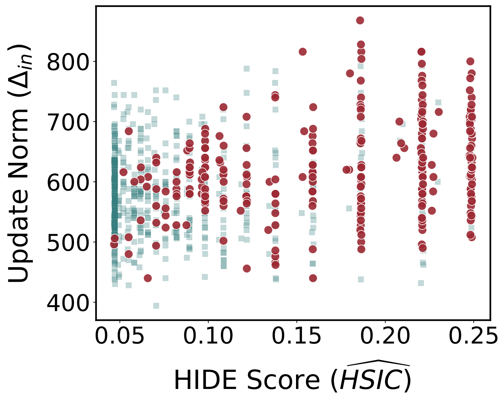
(c) SQuAD, PCC: 0.302
