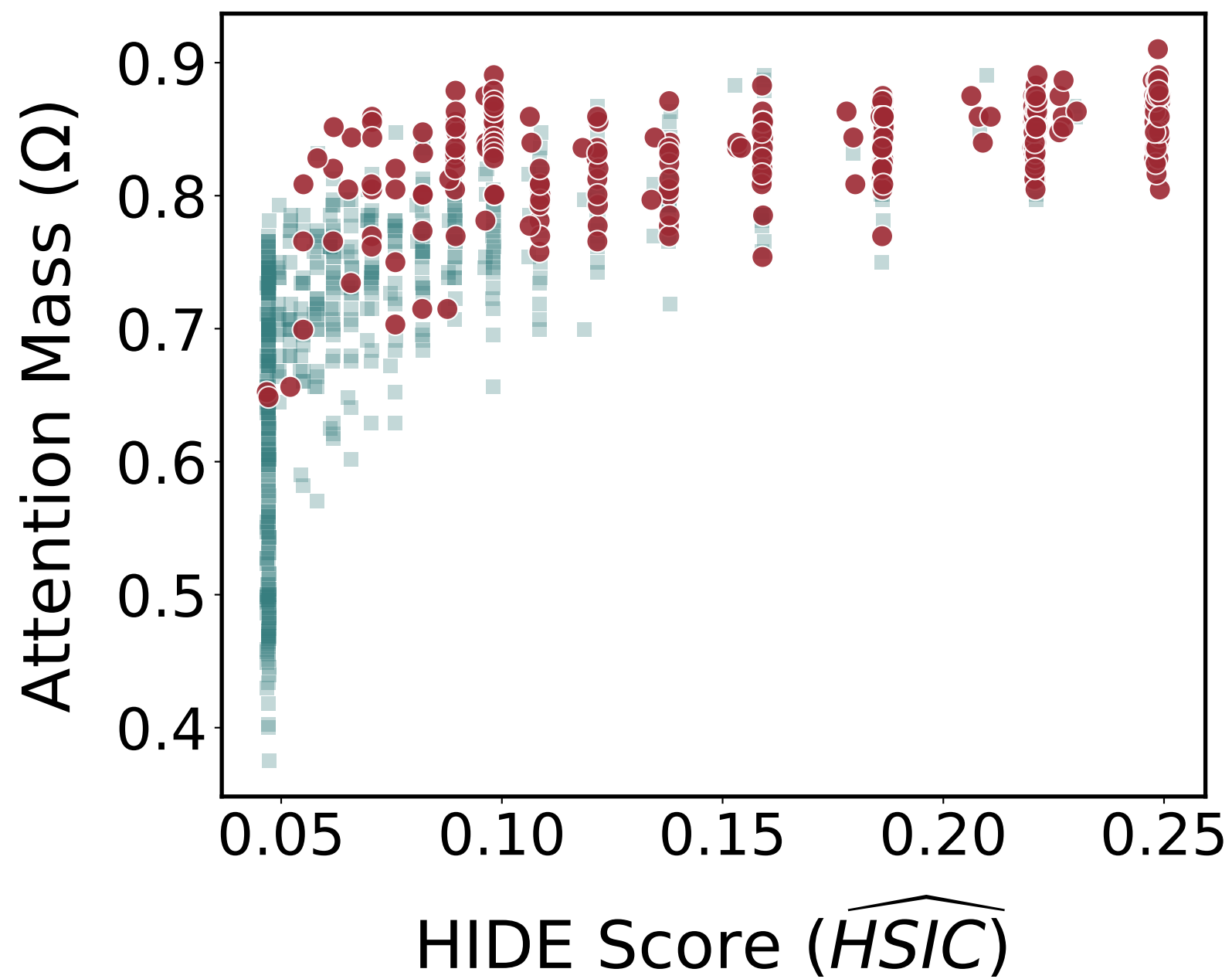
(a) SQuAD, PCC: 0.703
