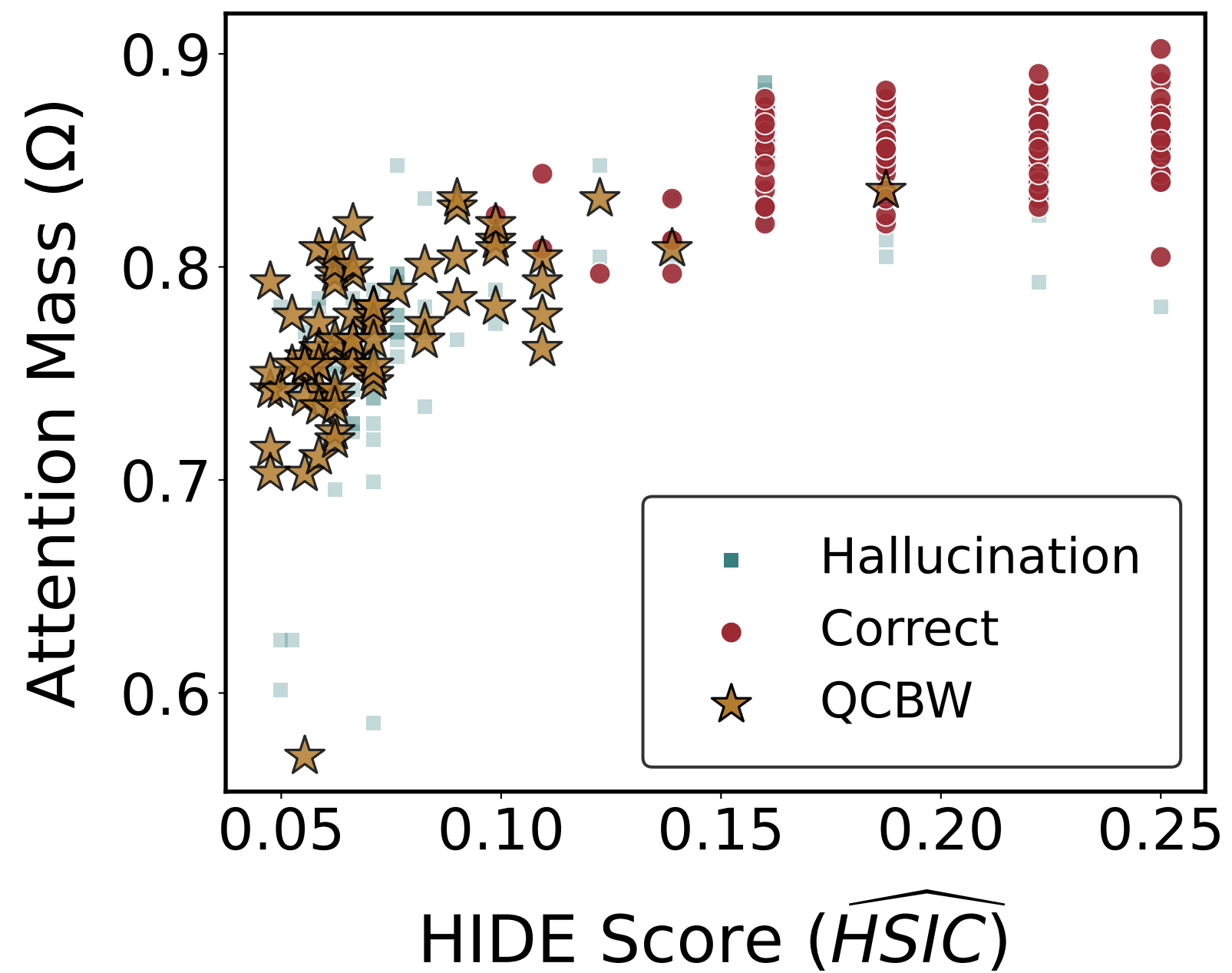
(b) NQ, PCC: 0.805
