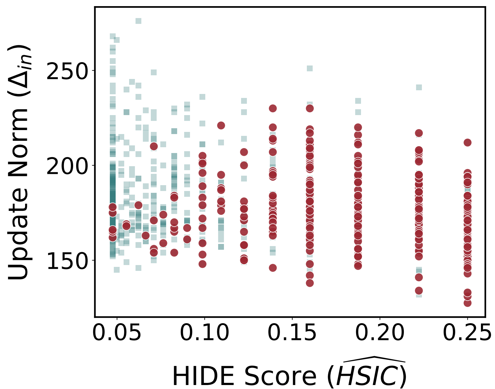
(c) SQuAD, PCC: -0.207
