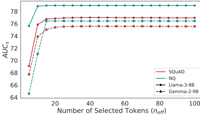
Figure 5: Historical token-budget ablation on SQuAD and NQ using Llama-3-8B and Gemma-2-9B. The horizontal axis gives the configured selected-token budget; the vertical axis is AUC_s (sentence-similarity correctness threshold 0.9, higher is better). The actual selected count may be smaller for short answers. Curves level off around 15–20 tokens; this is an observed sensitivity result, not proof of a structural mechanism.
