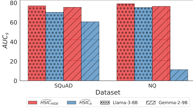
Figure 8: Historical estimator comparison for Llama-3-8B and Gemma-2-9B on SQuAD and NQ. Bars compare the adapted HIDE estimator with biased HSIC using AUC_s (sentence-similarity correctness threshold 0.9, higher is better). The comparison concerns the configured estimators; the selected-token-count control in Appendix F limits attributing the difference solely to nonlinear dependence.
