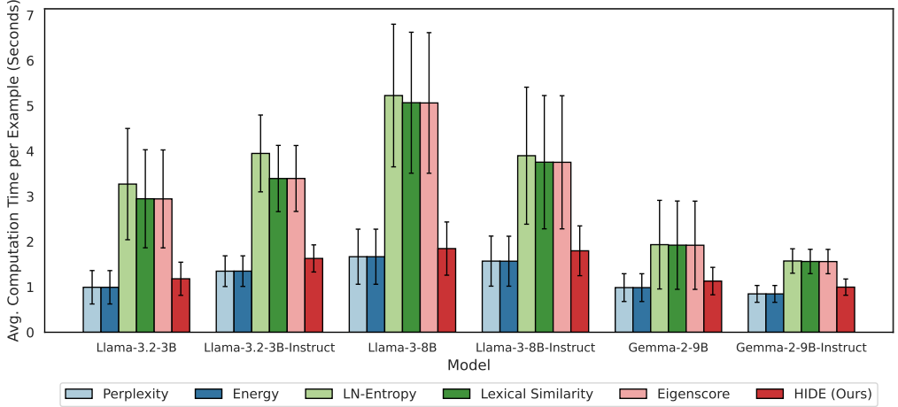
Figure 3: Historical baseline architectural comparison under standard HuggingFace inference on an A100-SXM4-80GB: average per-example latency for six models, averaged across the original RACE, SQuAD, NQ, and TriviaQA evaluation instances. HIDE uses one generation; the multi-pass methods use five outputs per prompt. HIDE includes generation, keyword extraction, and score computation. These original measurements are retained separately from the new paired base/HIDE experiment in Table 6; their hardware/protocol and averaging populations differ. The reported approximately 51% reduction pertains only to this baseline comparison and is neither an optimized-serving measurement nor a lower bound.
