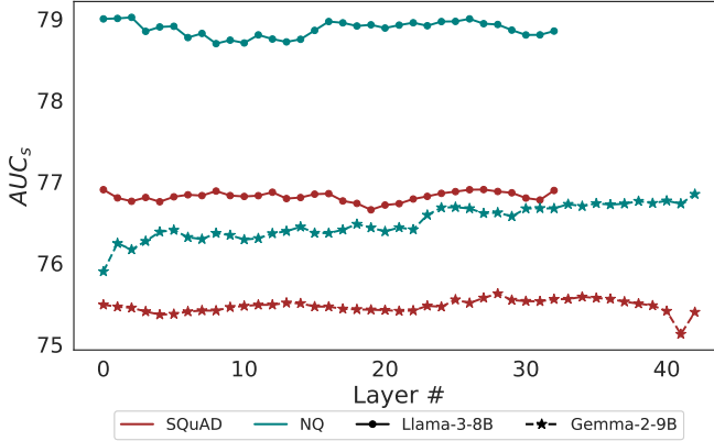
Figure 6: Historical layer ablation for Llama-3-8B and Gemma-2-9B on SQuAD and NQ. The horizontal axis gives the selected layer and the vertical axis AUC_s (sentence-similarity correctness threshold 0.9, higher is better). Curves show limited variation in these experiments; this does not identify distributed causal mechanisms.
