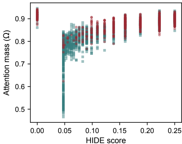
(a) SQuAD; PCC = 0.560
