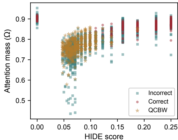
(b) NQ; PCC = 0.648
