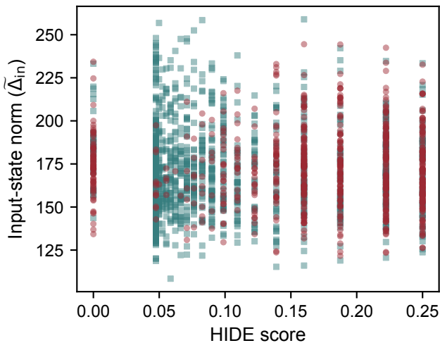
(c) SQuAD; PCC = 0.003
