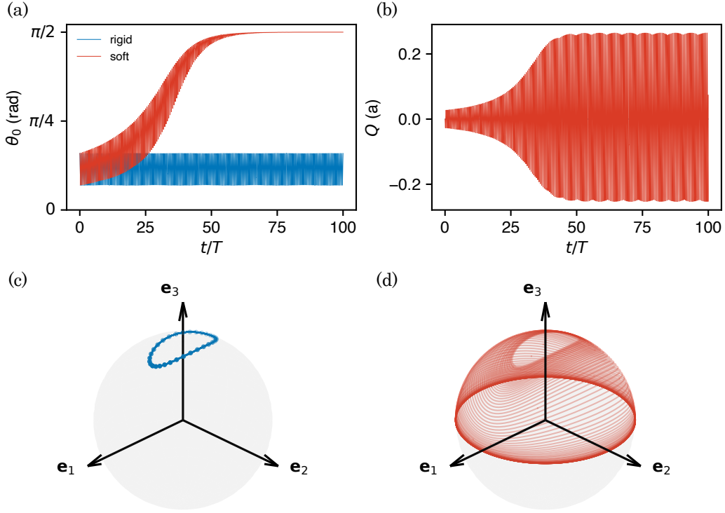
FIG. 9. Jeffery's orbits of a soft dumbbell.
