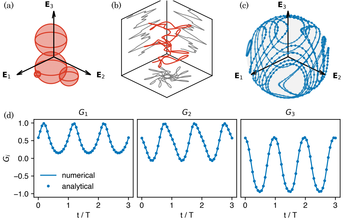
FIG. 4. Sinking dynamics of a chiral rigid body. (a) Geometry of the body, with body's frame (\mathbf{E}_1, \mathbf{E}_2, \mathbf{E}_3) centered on the center of mass (identical to the hydrodynamic center of mobility). (b) Example of trajectory \mathbf{r}_0 of the center of mass in the laboratory frame (the vertical axis \mathbf{e}_3 is compressed by a factor 300). (c) Periodic orbits of the unit gravity vector \mathbf{G} in the body's frame (lines: simulation, dots: analytical solution). (d) Example of a periodic of orbits: the three components of \mathbf{G} are shown as a function of time.
