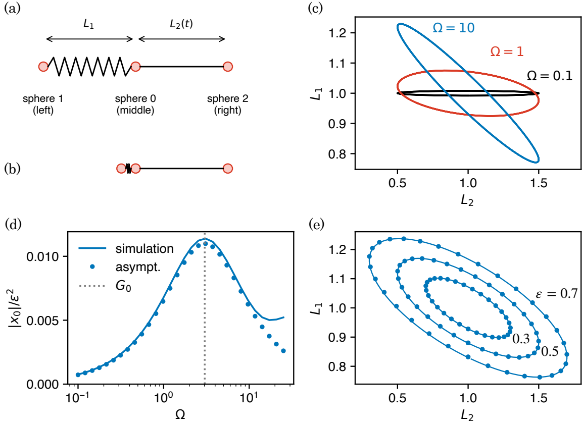
FIG. 8. Optimization of the three-sphere swimmer. (a) Default geometry with L_2 = 1 + \varepsilon \sin(t) , spring rest length l_1 = 1 , and sphere radius a_i = 0.05 . (b) Optimized geometry for free k , a_1 and l_1 . (c) Orbits of the swimmer in the L_2 - L_1 plane for different values of the dimensionless frequency \Omega = 2/k , with k the spring stiffness. (d) Swimming displacement over one period |x_0| as a function of \Omega , for the default geometry and \varepsilon = 0.1 (line: simulation, dots: analytical asymptotics in the limit of small \varepsilon ). (e) Orbits of the swimmer at optimal frequency \Omega = G_0 for different values of the forcing amplitude \varepsilon , as labelled.
