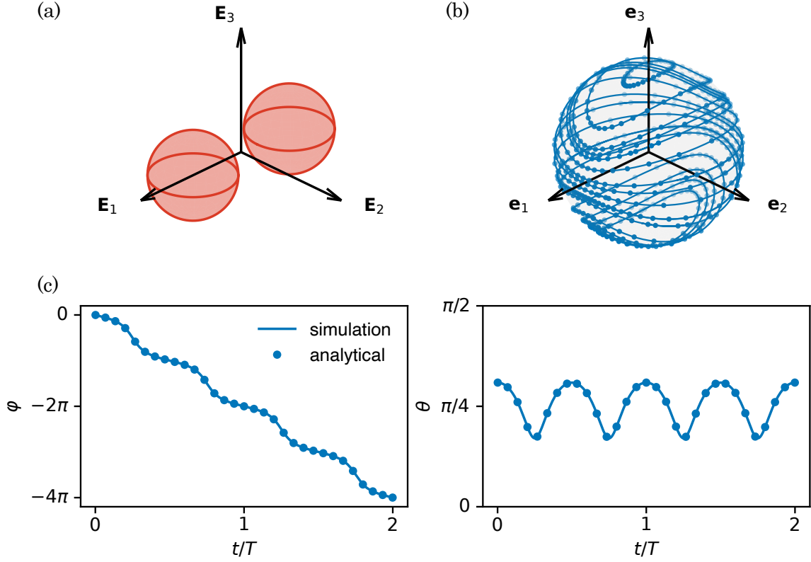
FIG. 7. Jeffery orbits of a rigid dumbbell in a pure shear flow of unit shear rate in the \mathbf{e}_1 - \mathbf{e}_2 plane: \mathbf{u}^\infty = [y, 0, 0] . (a) Geometry of the rigid body considered in the body's frame. (b) Jeffery periodic orbits of \mathbf{E}_1 in the laboratory's frame for different initial conditions (lines: simulation, dots: analytical solution). (c) Example of an orbit of \mathbf{E}_1 as a function of time in the spherical coordinate (r, \theta, \varphi) .
