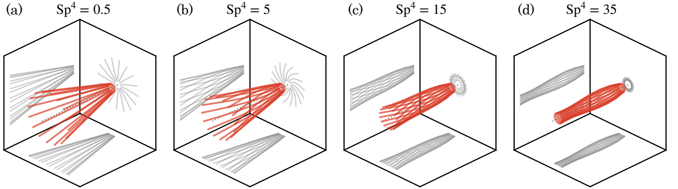
FIG. 6. Shape of a rotating flexible filament. The filament is made of N = 8 beads and is set at an angle \psi = 15^\circ with an offset of \delta_0/L = 0.05 with respect to the horizontal rotating axis. The only dimensionless number is the Sperm number Sp = L/L_\omega , with L_\omega = (K_b/\mu_\perp \omega)^{1/4} and \mu_\perp = 4\pi\mu/\ln(L/a) + 1/2 , the slider-body transverse drag.
