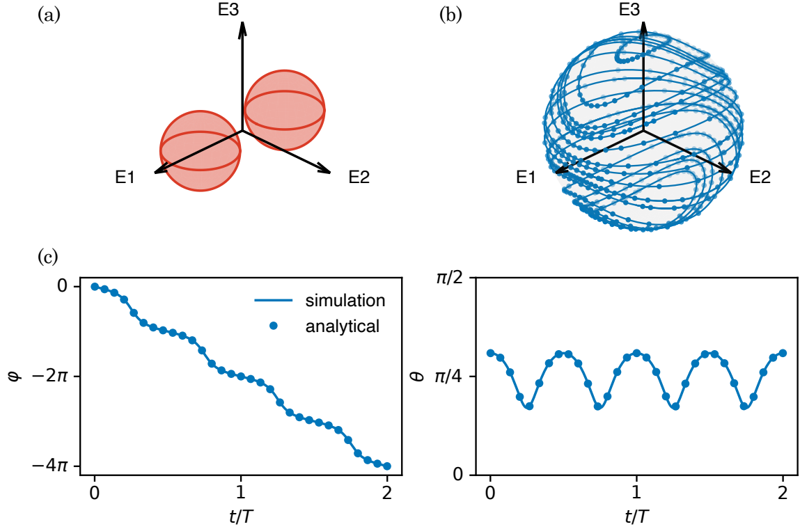
FIG. 7. Jeffery orbits of a rigid dumbbell in a pure shear flow of unit shear rate in the \mathbf{e}_1 - \mathbf{e}_2 plane: \mathbf{u}_0^\infty = [\mathbf{e}_2, 0, 0] . (a) Geometry of the rigid body considered in the body's frame. (b) Jeffery periodic orbits of \mathbf{E}_1 in the laboratory's frame for different initial conditions (lines: simulation, dots: analytical solution). (c) Example of an orbit of \mathbf{E}_1 as a function of time in the spherical coordinate (r, \theta, \phi) .
