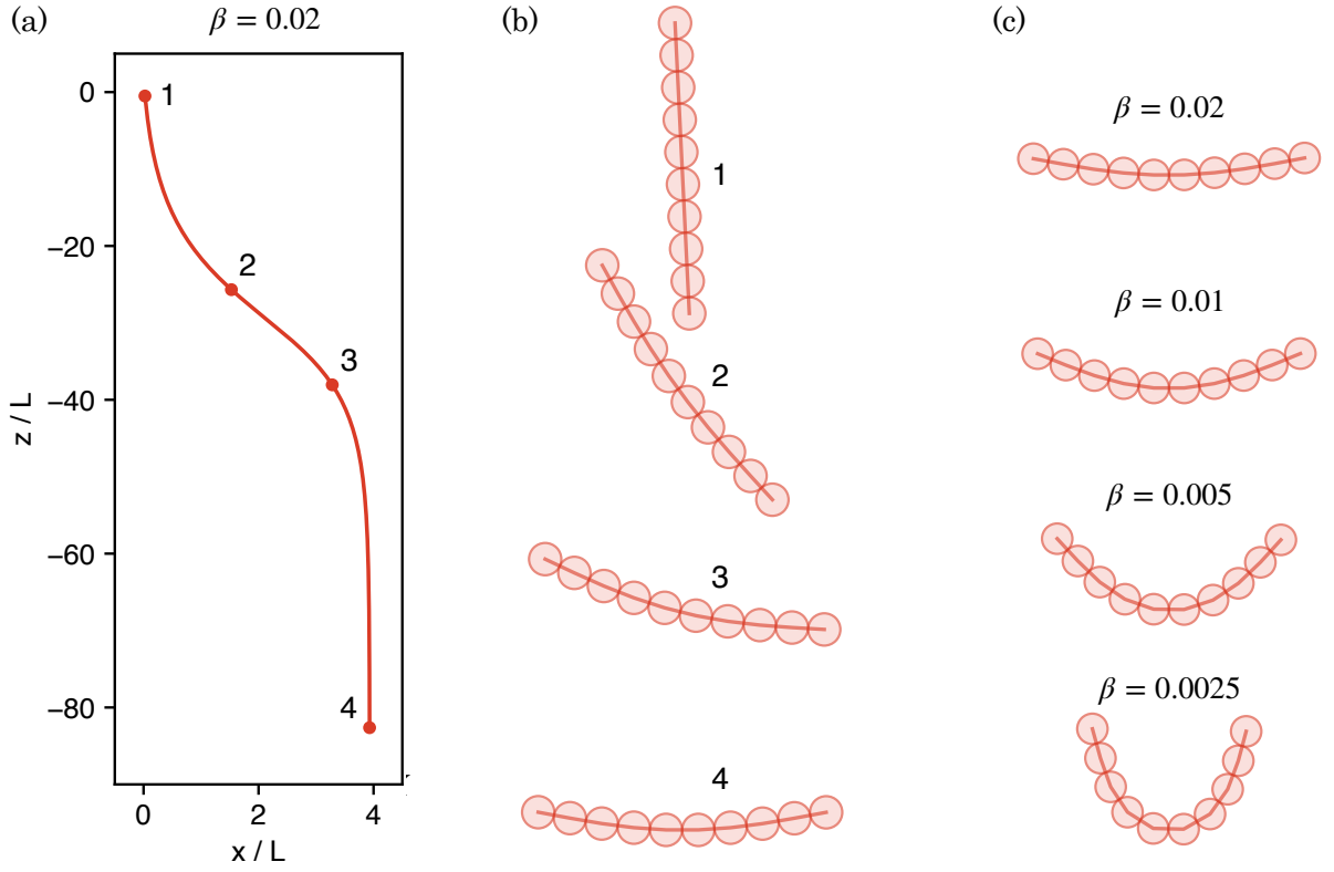
FIG. 5. Sinking dynamics of a flexible fiber ( N = 10 beads of radius a ). The torsional spring stiffness is k = K_b/2a , with K_b the equivalent beam rigidity and dimensionless rigidity \beta = K_b/F_\perp L^2 , with F_\perp = Nmg the total weight. (a) For an initial angle of \pi/32 with respect to the vertical, the graph shows the position of the center of mass of the fiber in the laboratory frame. (b) Snapshots showing the deformation of the fiber along the trajectory shown in (a). (c) Final shape for fiber of decreasing rigidity as labelled.
