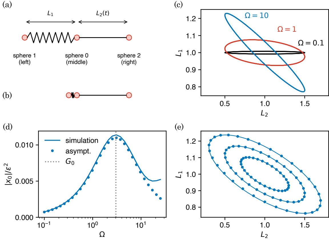
FIG. 8. Optimization of the three-sphere swimmer. (a) Default geometry with L_2 = l_2(1 + \varepsilon \sin(\omega t)) , spring rest length l_1 = l_2 , and sphere radius a_i = 0.05l_2 . (b) Optimized geometry for fixed a_0 = a_2 = 0.05 . (c) Orbits of the swimmer in the L_2 - L_1 plane for different values of the dimensionless frequency \Omega = \omega\mu(l_1 + l_2)/k , with k the spring stiffness. (d) Swimming displacement over one period |x_0| as a function of \Omega , for the default geometry and \varepsilon = 0.1 (line: simulation, dots: analytical asymptotics in the limit of small \varepsilon ). (e) Orbits of the swimmer at optimal frequency \Omega = G_0 for different values of the forcing amplitude \varepsilon , as labelled.
