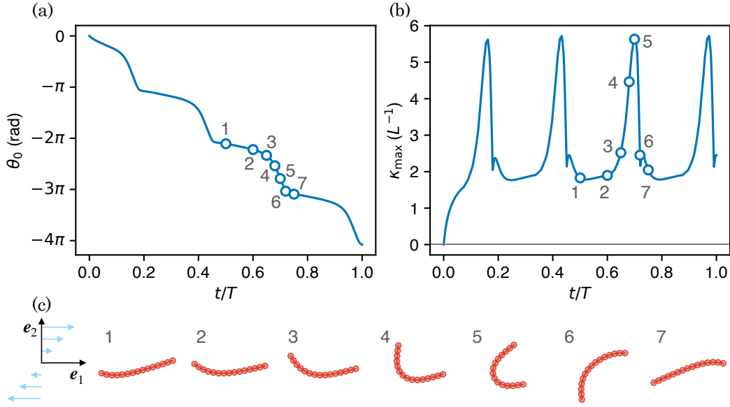
FIG. 7. Flexible fiber tumbling in pure shear flow. (a) Orientation angle \theta_0 around \mathbf{e}_3 of the leftmost sphere as a function of time, normalised by the Jeffery's period of the rigid assembly. (b) Maximum curvature of the fiber in units of length as a function of time. The horizontal grey line shows the intrinsic curvature of the fiber \kappa_0 = 0.01/L . (c) Snapshots of the fiber deformation as labelled in (b).
