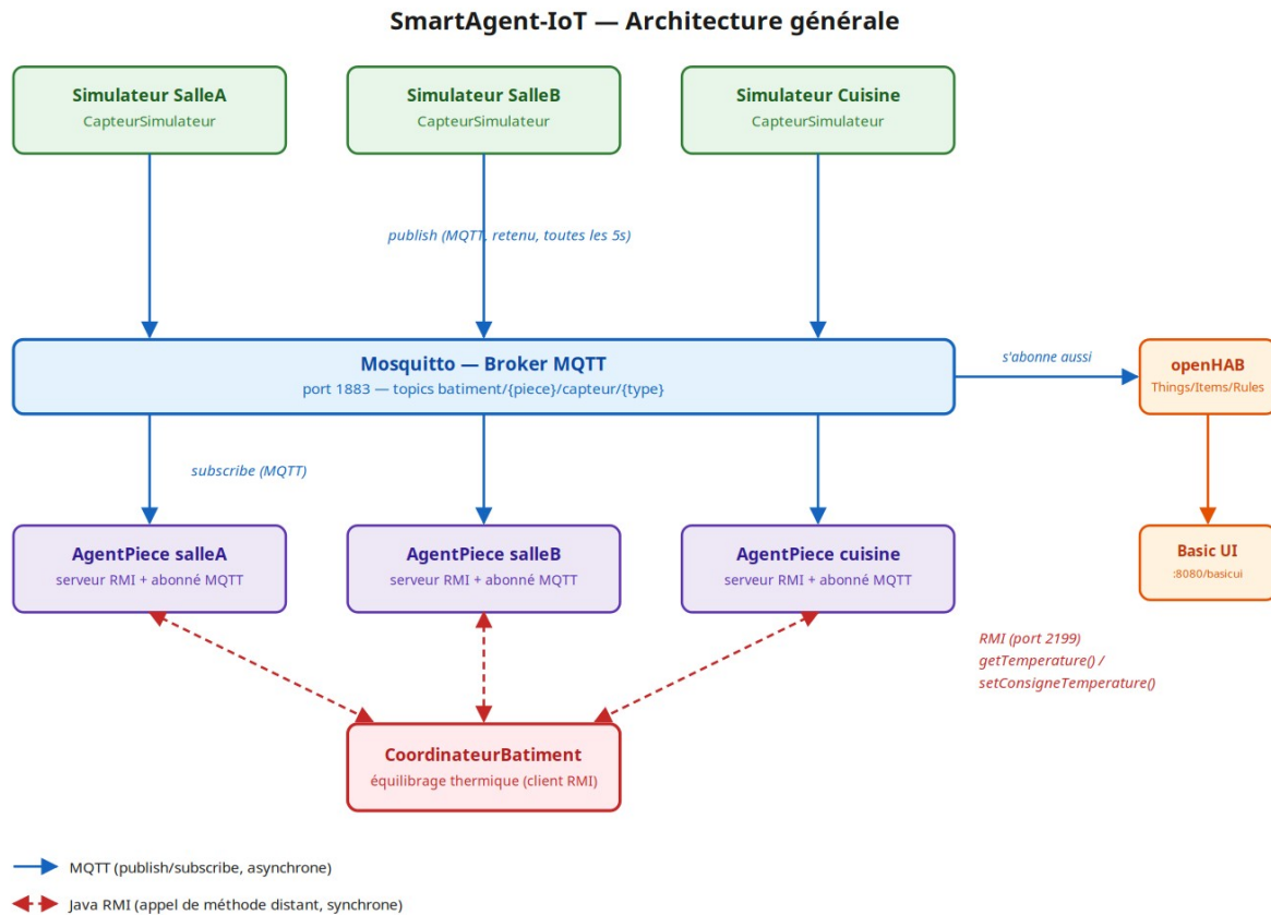
Figure 1 — Architecture generale de SmartAgent-IoT (capteurs, broker MQTT, agents RMI, coordinateur, openHAB)
