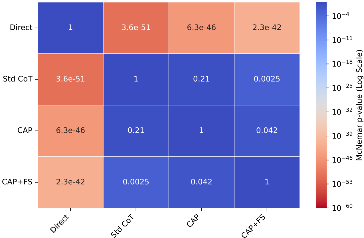
Statistical Significance Matrix (DeepSeek-Chat)
