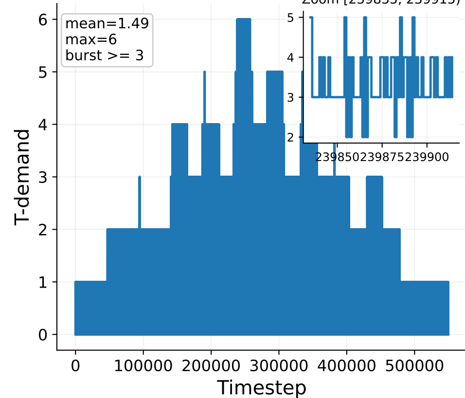
QFT n=8: Workload Characterization
