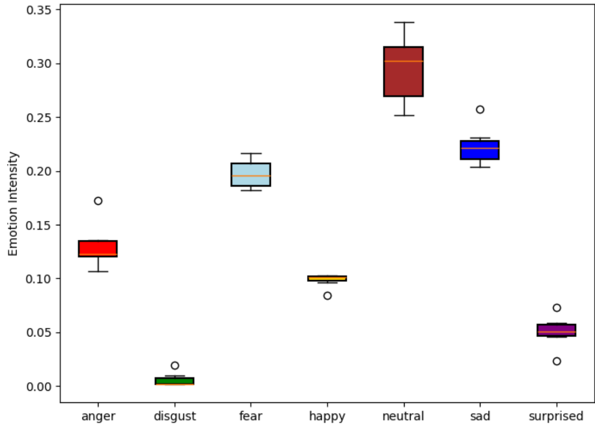
Box Plot for Session test
