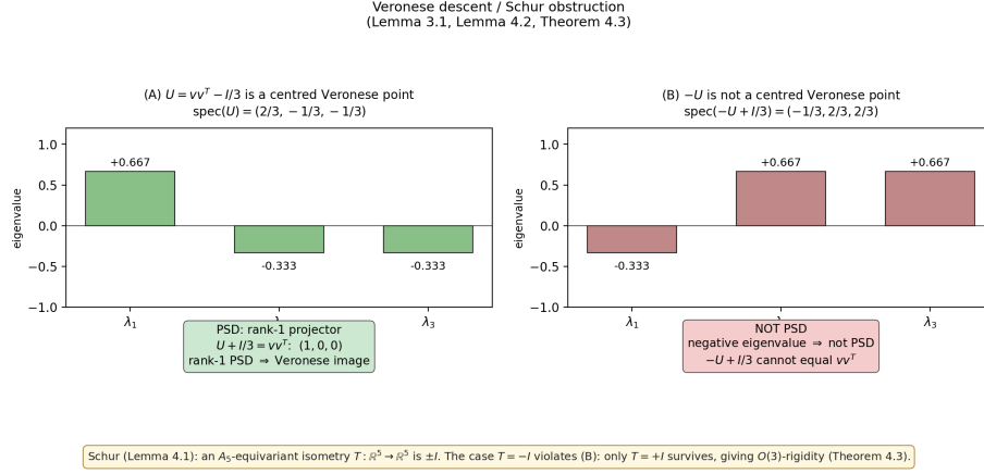
Figure 3: Figure 3. Veronese descent / Schur obstruction (Lemmas 3.1, 4.2, Theorem 4.3). (A) Spectrum of a Veronese image U = vv^T - I/3 : (2/3, -1/3, -1/3) . The shift U + I/3 has spectrum (1, 0, 0) , i.e. is a rank-1 PSD projector. (B) Spectrum of -U + I/3 : (-1/3, 2/3, 2/3) , which contains a negative eigenvalue, so -U + I/3 cannot be a rank-1 PSD projector. Schur’s lemma forces an A_5 -equivariant isometry T: \mathbb{R}^5 \rightarrow \mathbb{R}^5 to be \pm I ; the case T = -I would map Veronese-image points off the Veronese surface, so only T = +I survives — giving O(3) -rigidity (Theorem 4.3).
