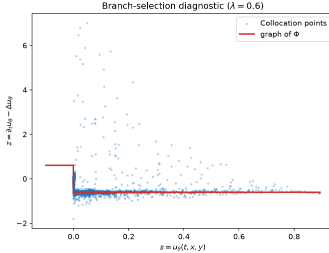
Figure 8: Branch-selection diagnostic ( \lambda = 0.6 ): empirical cloud of (u_\theta, \partial_t u_\theta - \Delta u_\theta) at 4000 post-training collocation points (blue dots), overlaid on the graph of \Phi (red). Points with s \gtrsim 0.05 cluster tightly on the branch z = -0.6 ; no points appear with s < 0 (sign preservation by the relay flow); the vertical scatter near s \approx 0 traces the extinction front, where the discontinuity of \Phi limits pointwise accuracy.
