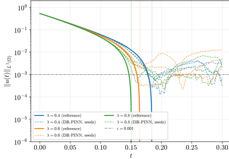
Figure 12: Reference extinction and DR-PINN threshold-crossing behaviour across \lambda \in \{0.4, 0.6, 0.8\} . Solid lines show the reference solutions and dashed lines the three DR-PINN seeds for each \lambda (blue: 0.4, orange: 0.6, green: 0.8); the dash-dotted horizontal line marks the threshold 10^{-3} . Curves are clipped below 10^{-6} for readability. The reference solutions extinguish exactly, whereas most DR-PINN curves cross the threshold only transiently and retain a small nonzero post-extinction norm.
