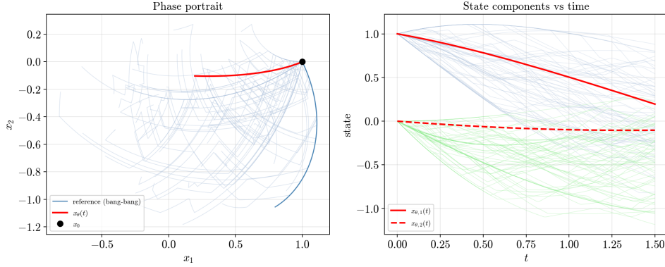
Figure 3: Phase portrait (left) and state components versus time (right) for the trained trajectory x_{\theta}(t) , compared with the reference reachable tube \mathcal{R}(t) (304 trajectories, light blue) and one representative bang-bang extremal (dark blue).
