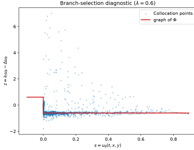
Figure 11: Branch-selection diagnostic ( \lambda = 0.6 ): empirical cloud of (u_\theta, \partial_t u_\theta - \Delta u_\theta) at 4000 post-training collocation points (blue dots), overlaid on the graph of \Phi (red). Points with s \gtrsim 0.05 cluster tightly on the branch z = -0.6 ; no points appear with s < 0 (sign preservation by the relay flow); the vertical scatter near s \approx 0 traces the extinction front, where the discontinuity of \Phi limits pointwise accuracy. The inset magnifies the neighborhood of the extinction front ( s close to 0).
