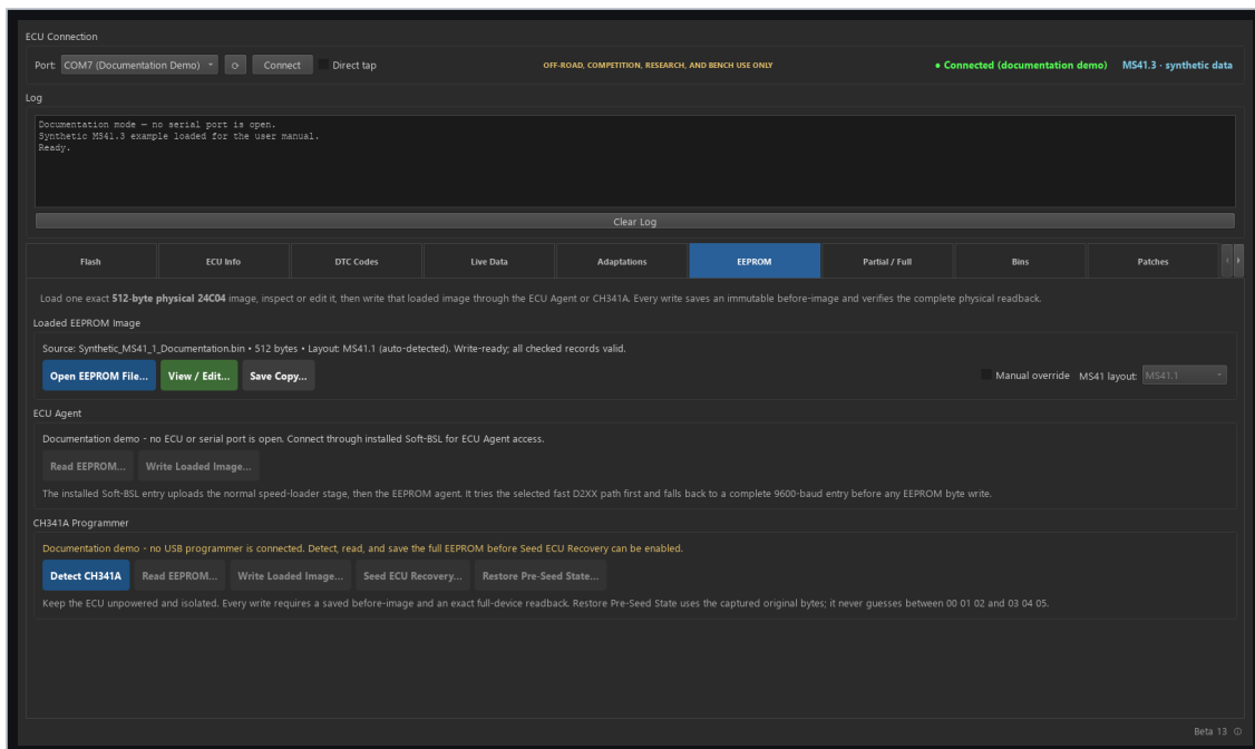
Loaded image, ECU Agent, and CH341A EEPROM workflows
