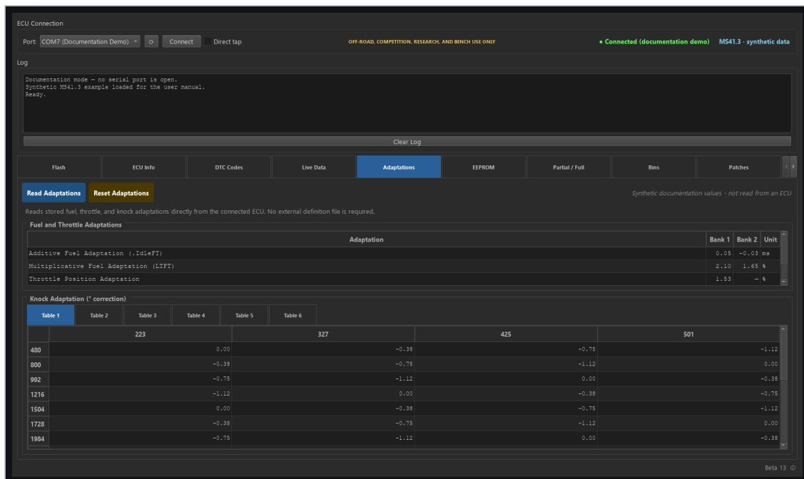
Stored fuel, throttle, and knock adaptations
