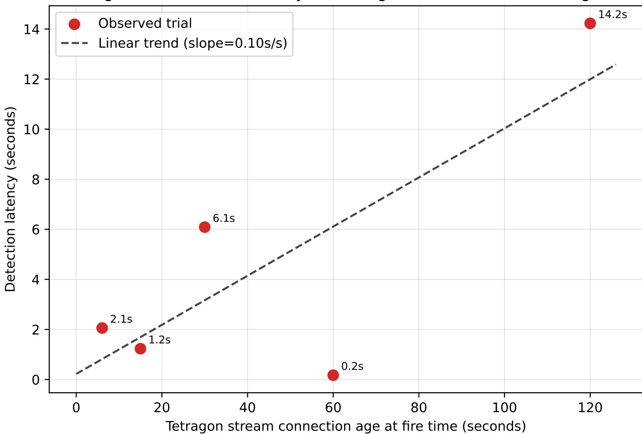
Fig. 7 — Detection Latency vs. Tetragon Stream Connection Age
