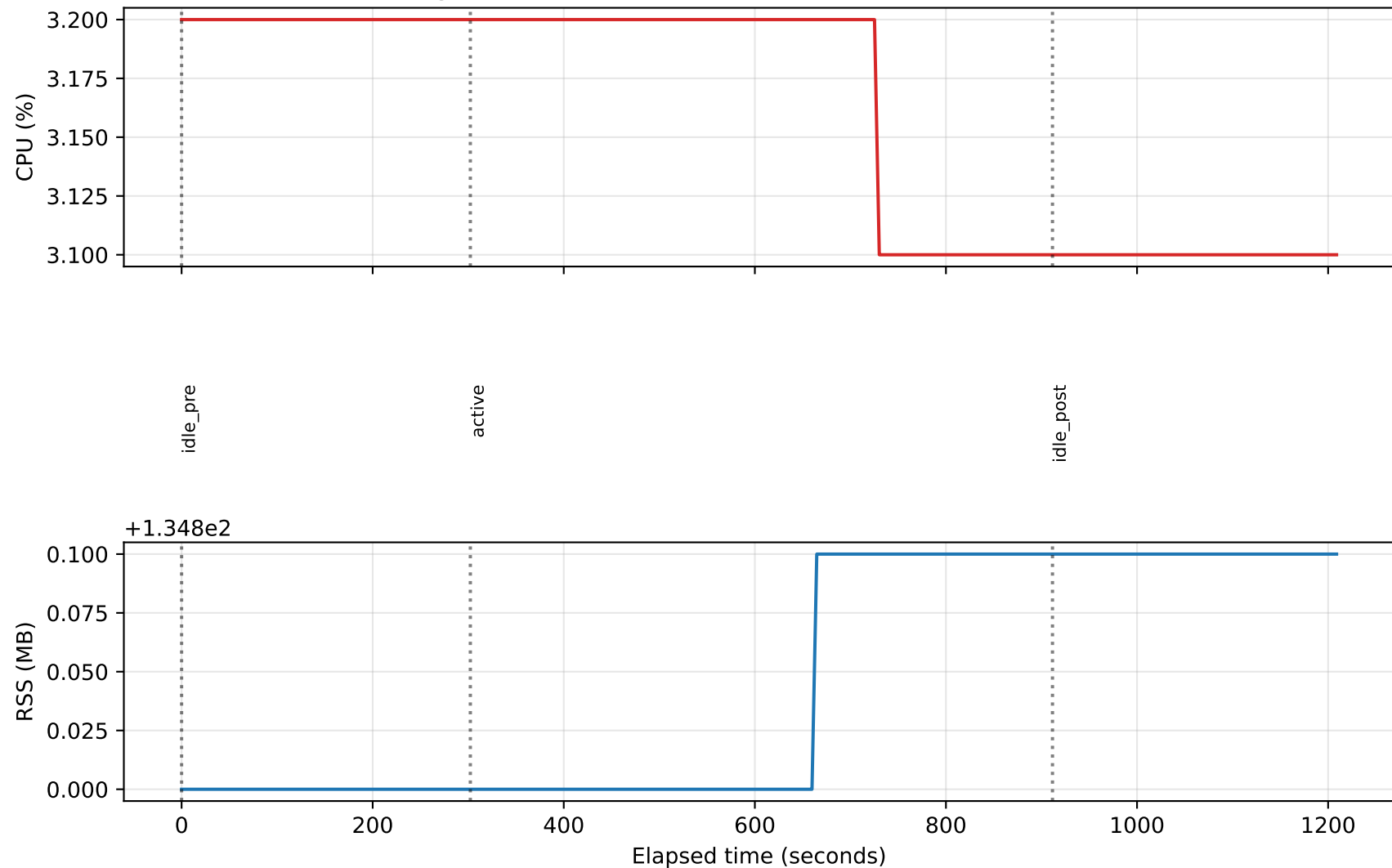
Fig. 9 — CAGE Server Resource Utilization Over Time
